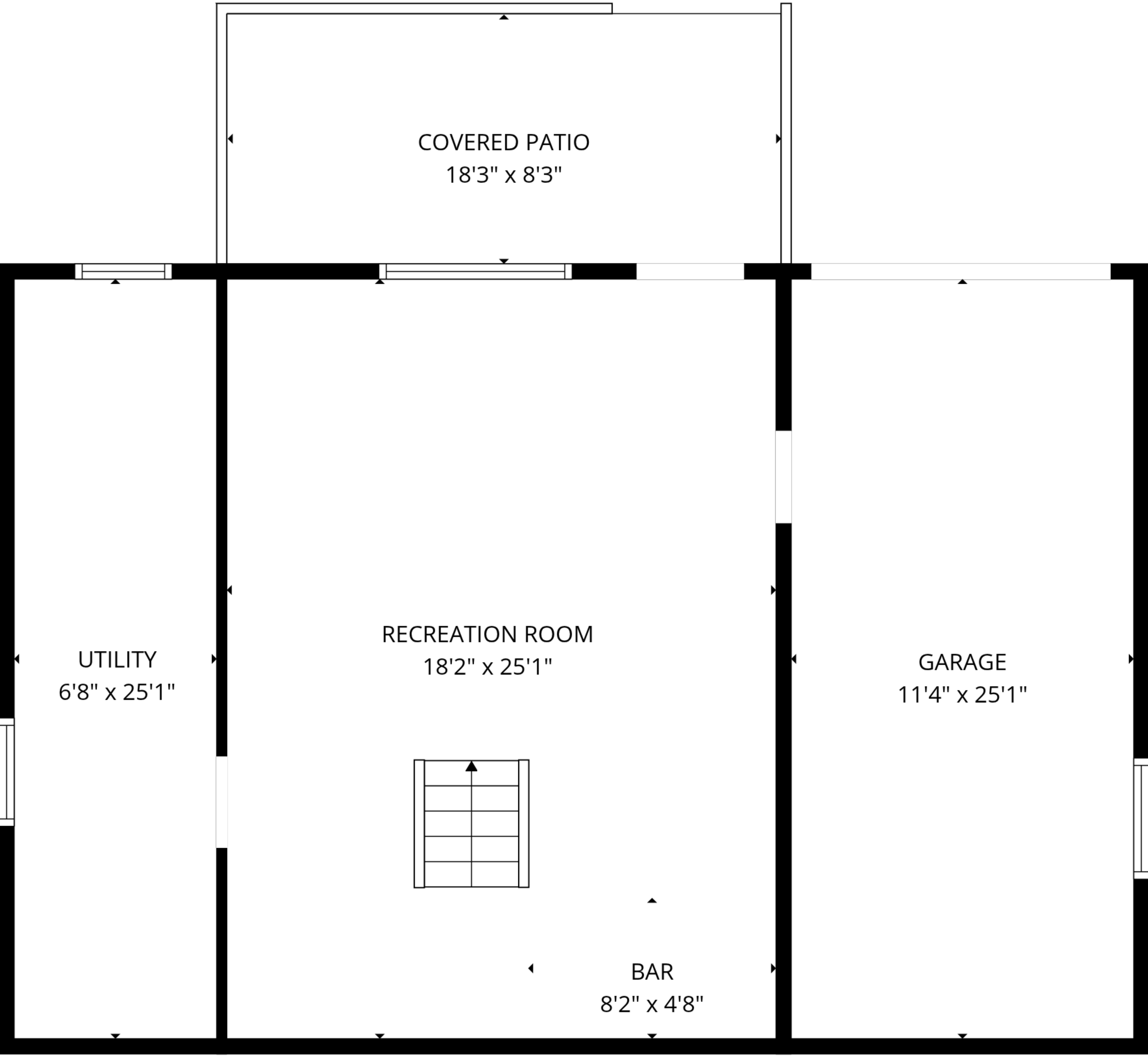
1st floor
