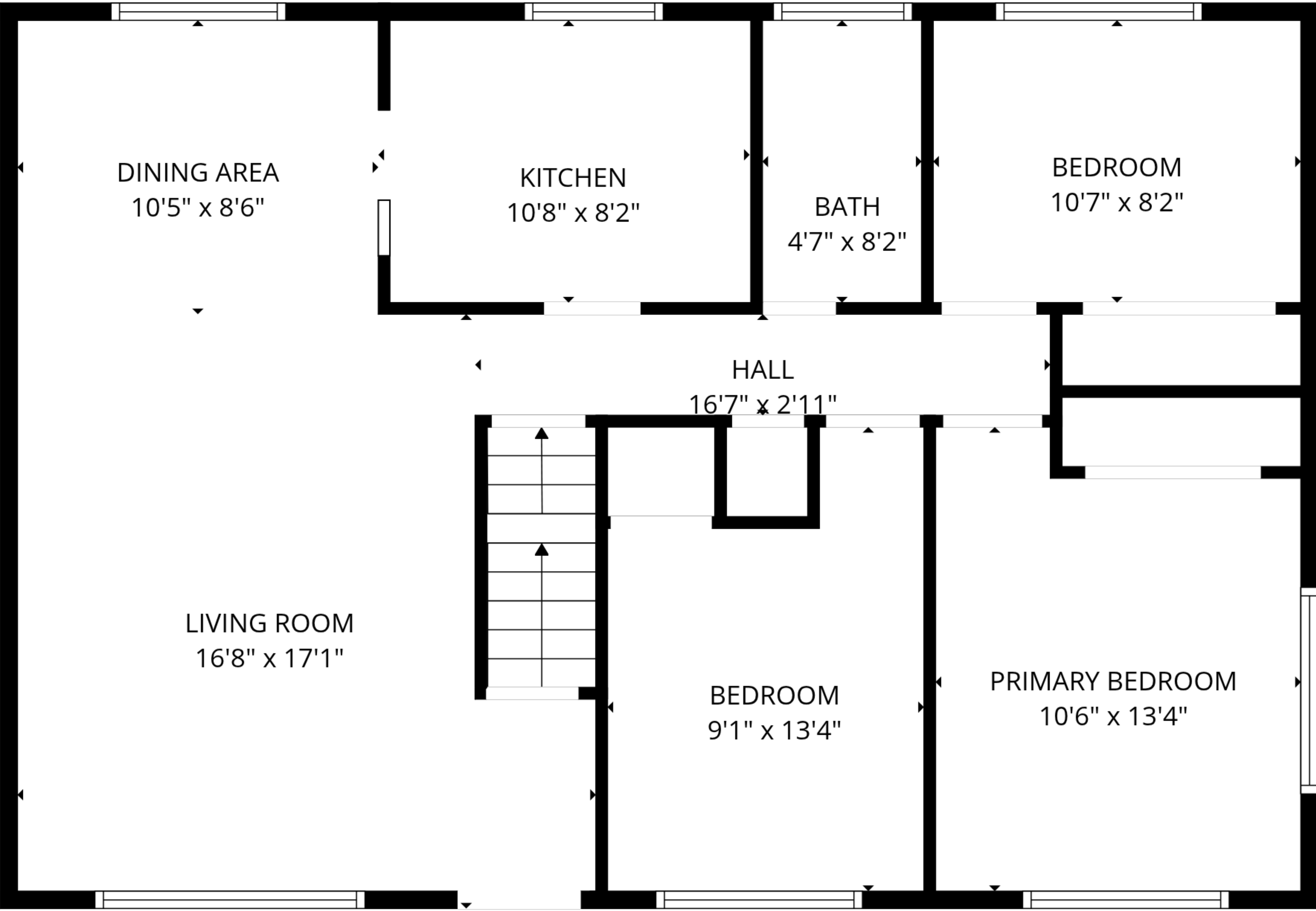
2nd floor
