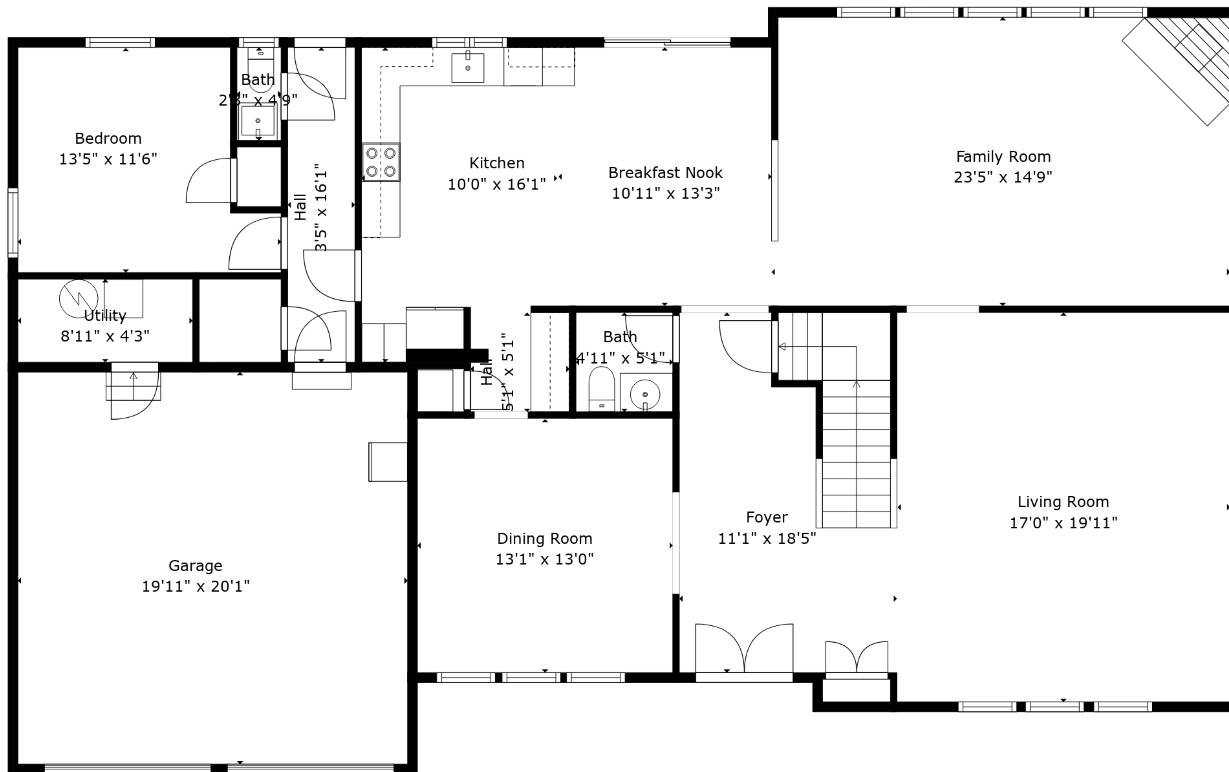
Floor 2
