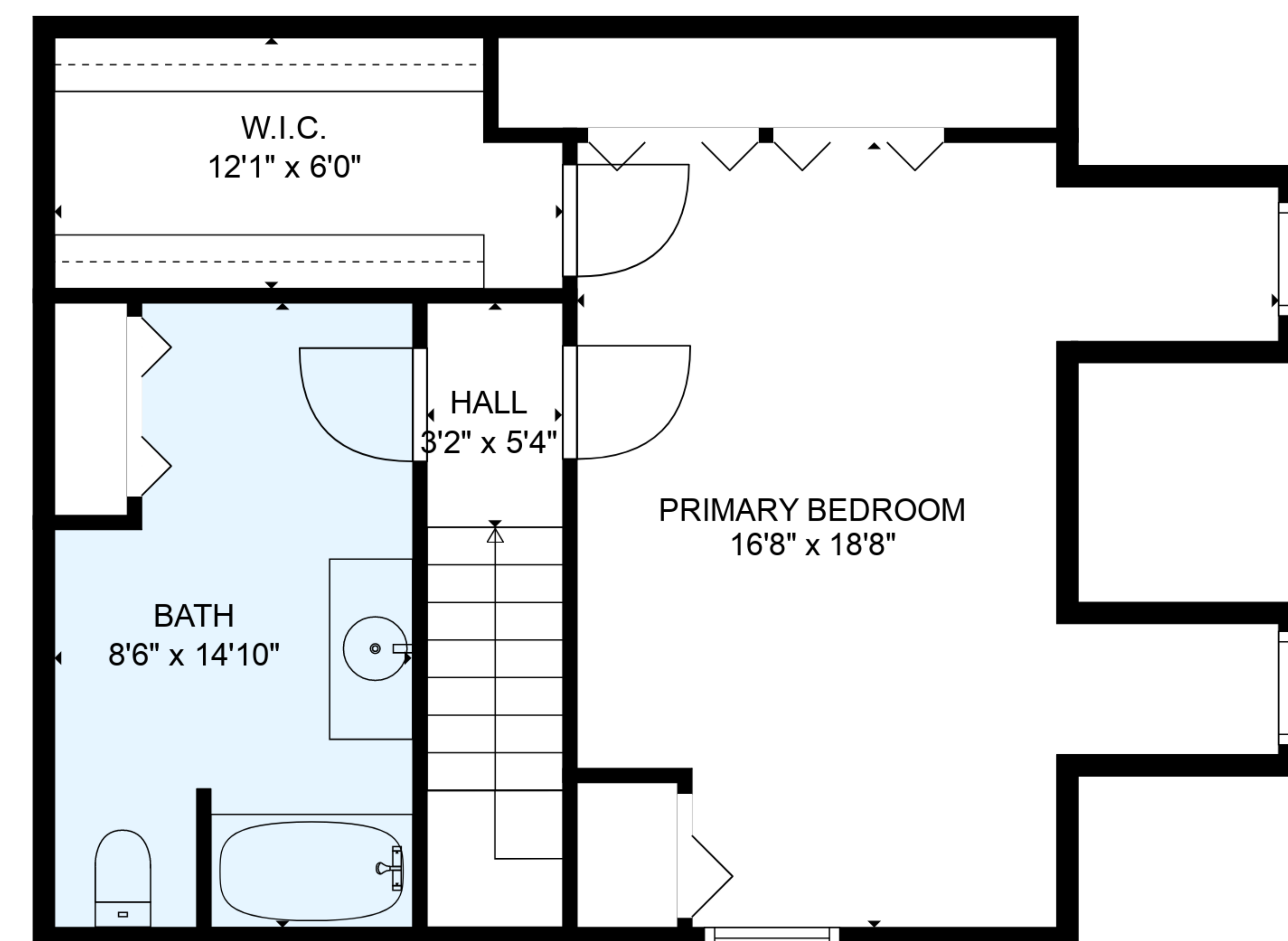
FLOOR 2
