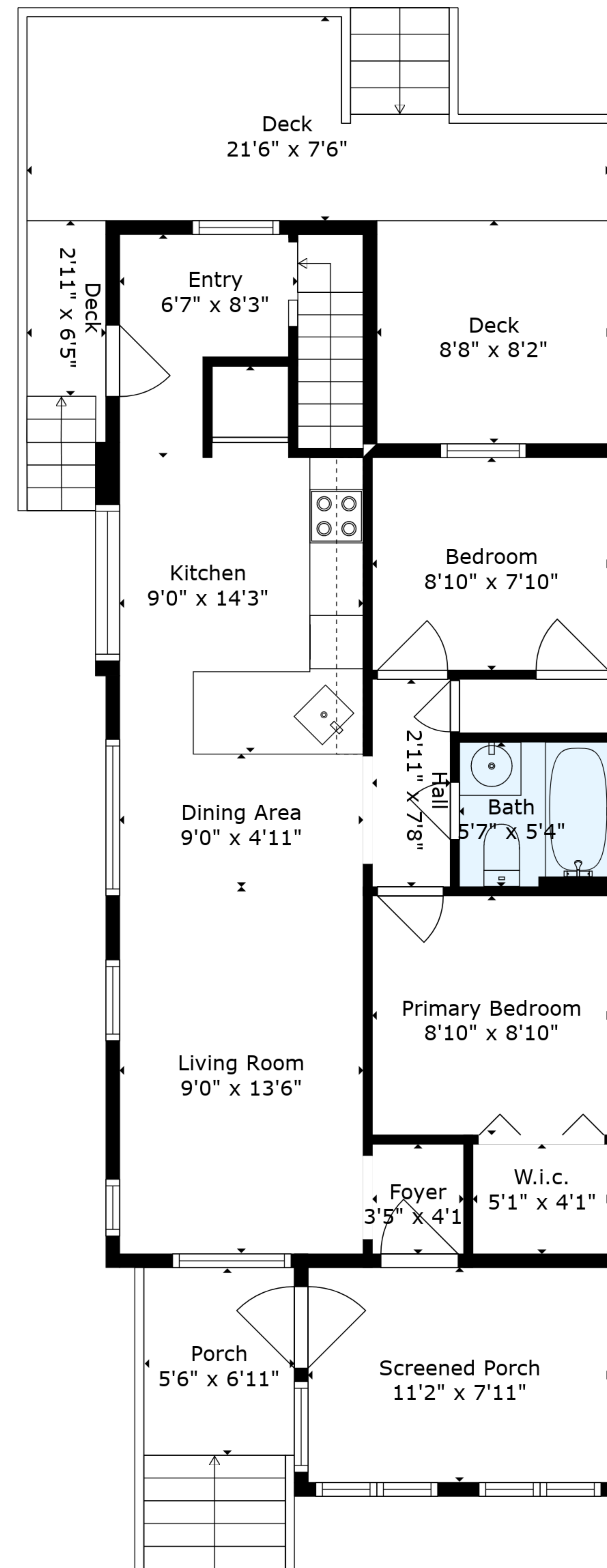
Floor 2
