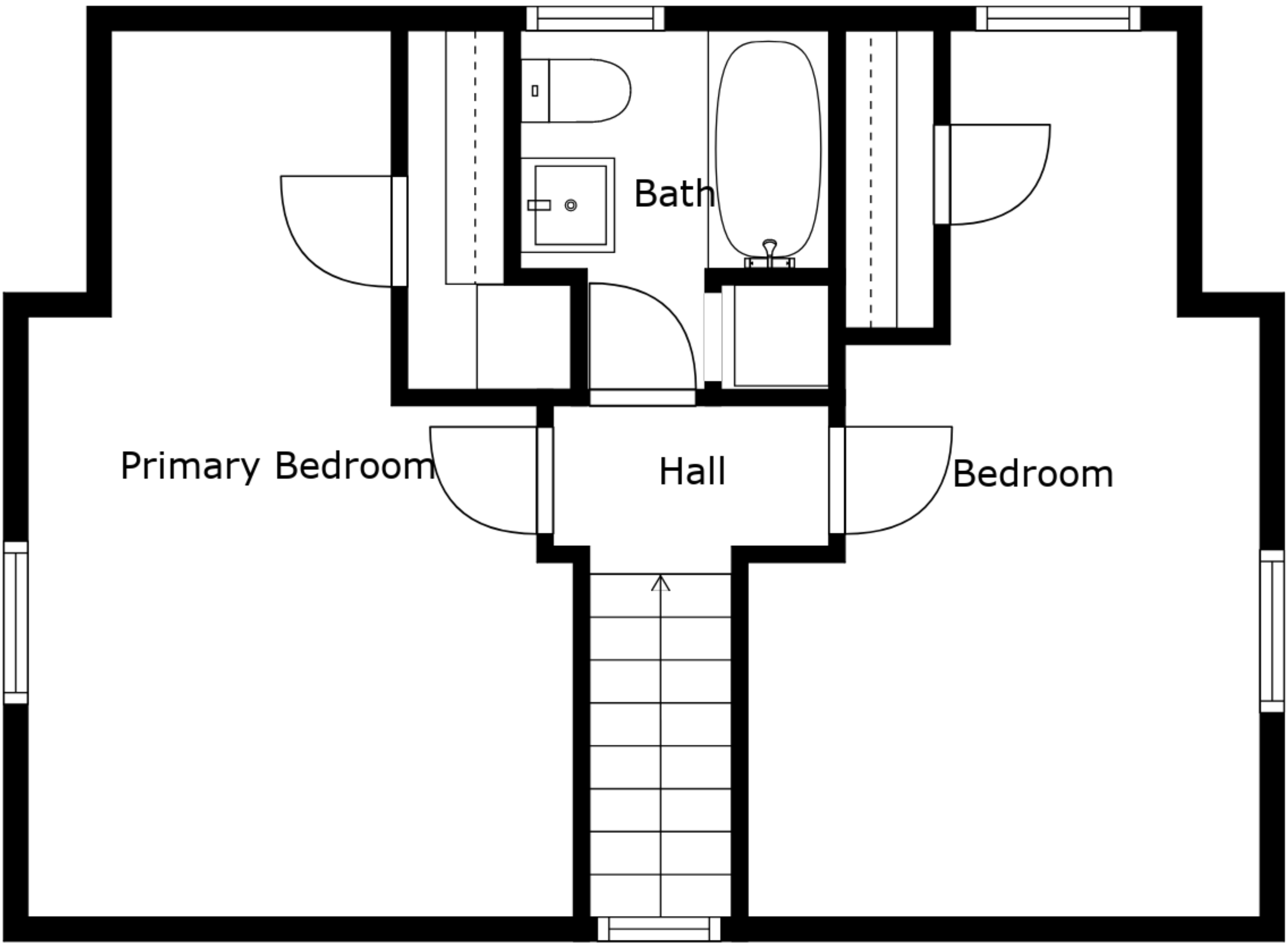
Floor 3
