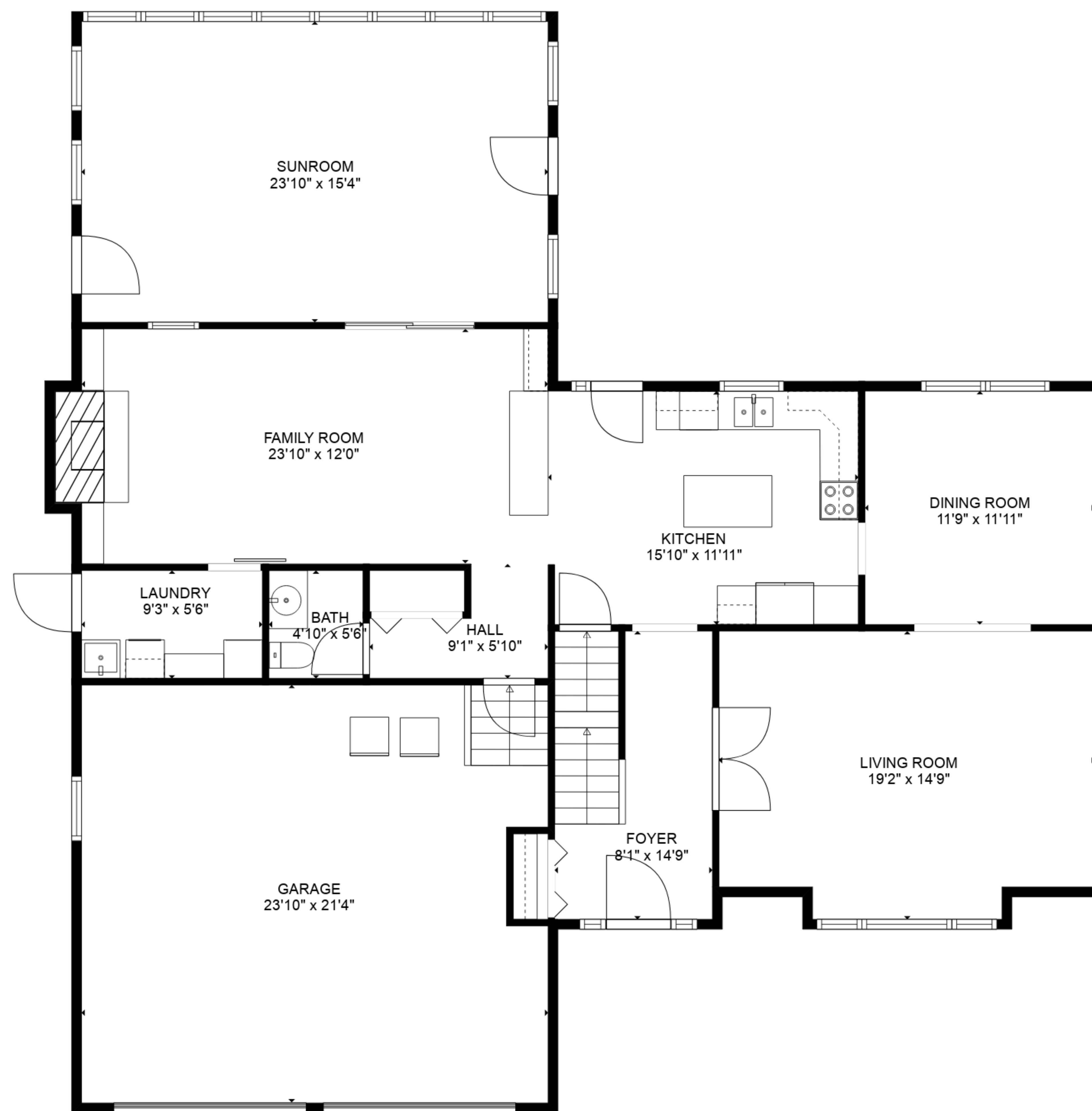
FLOOR 2
