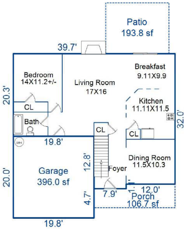
First Floor 1047.4 sf
