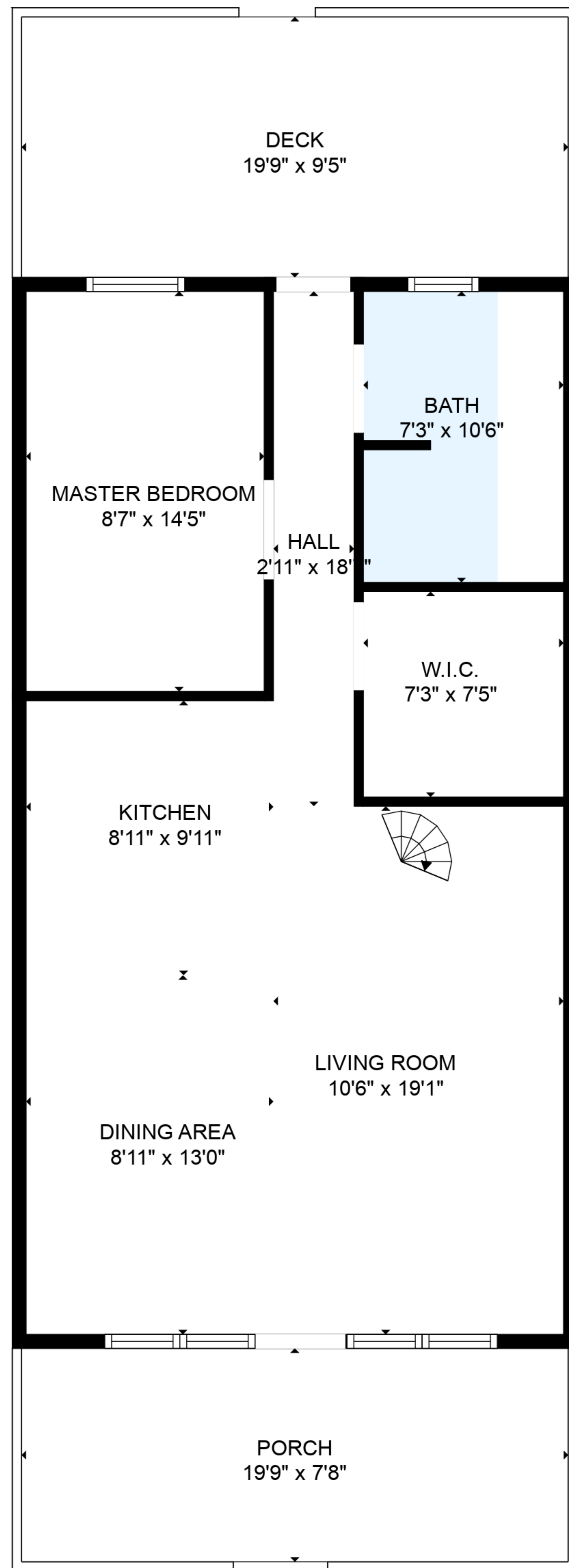
FLOOR 1
