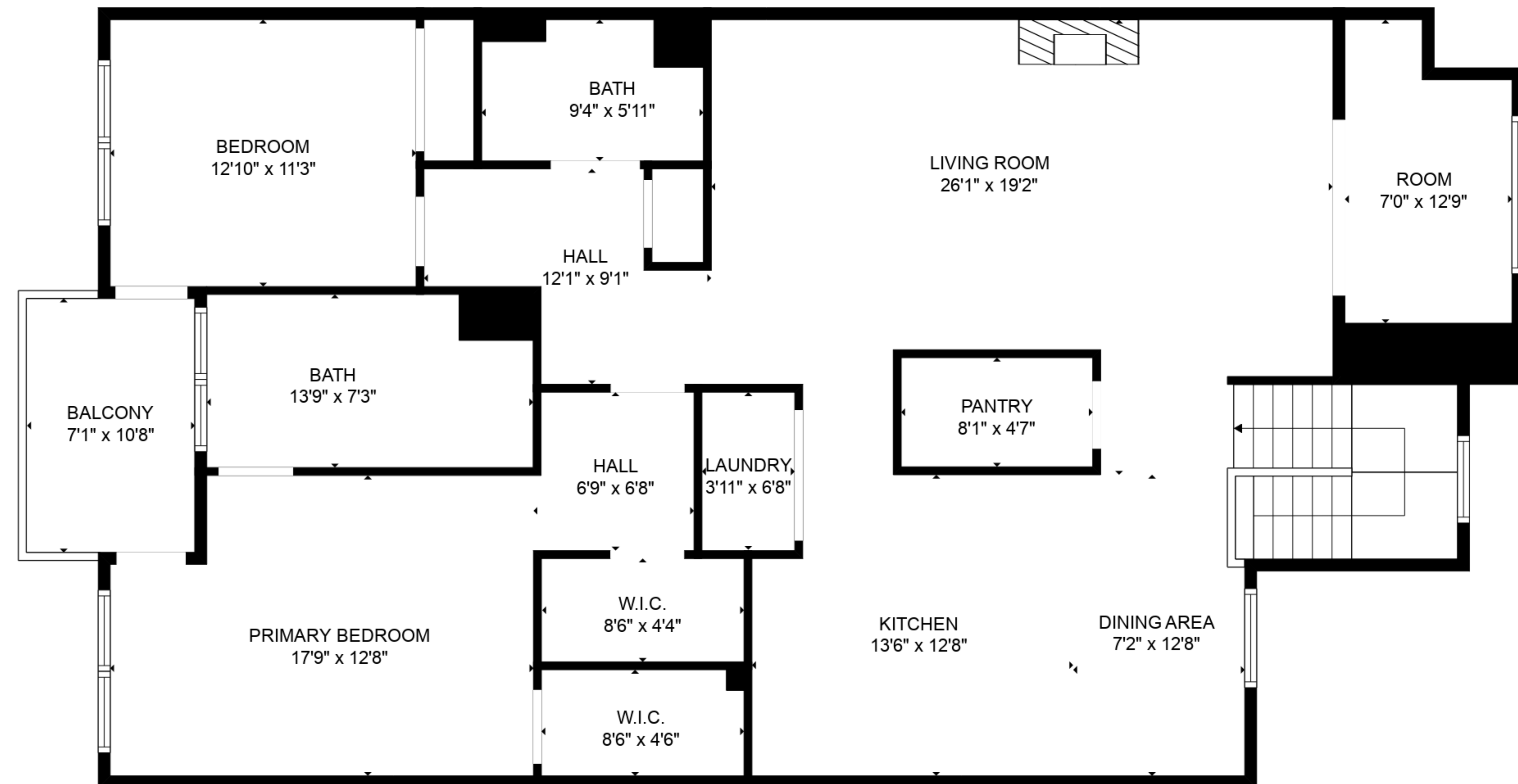
FLOOR 3
