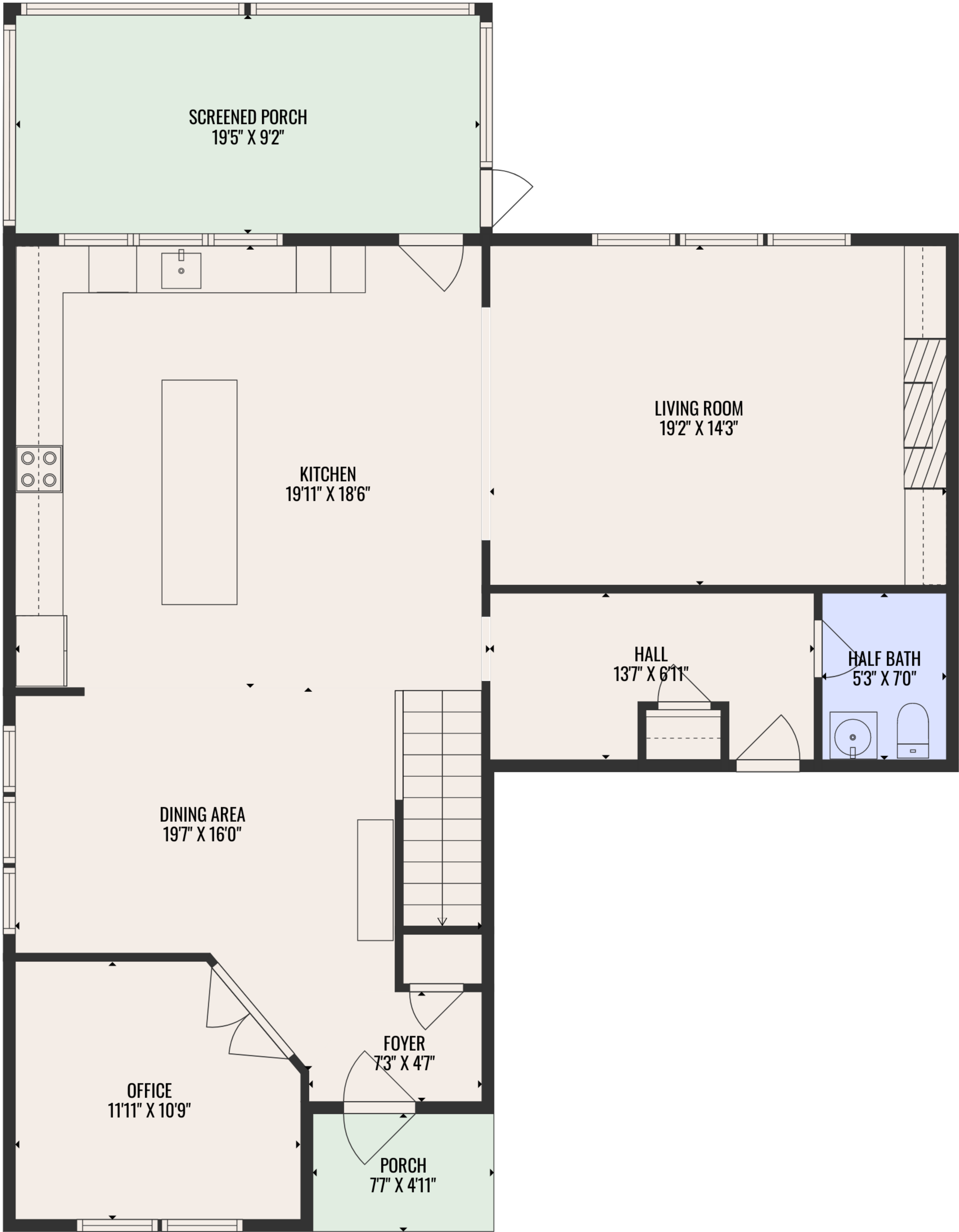
FLOOR 1
