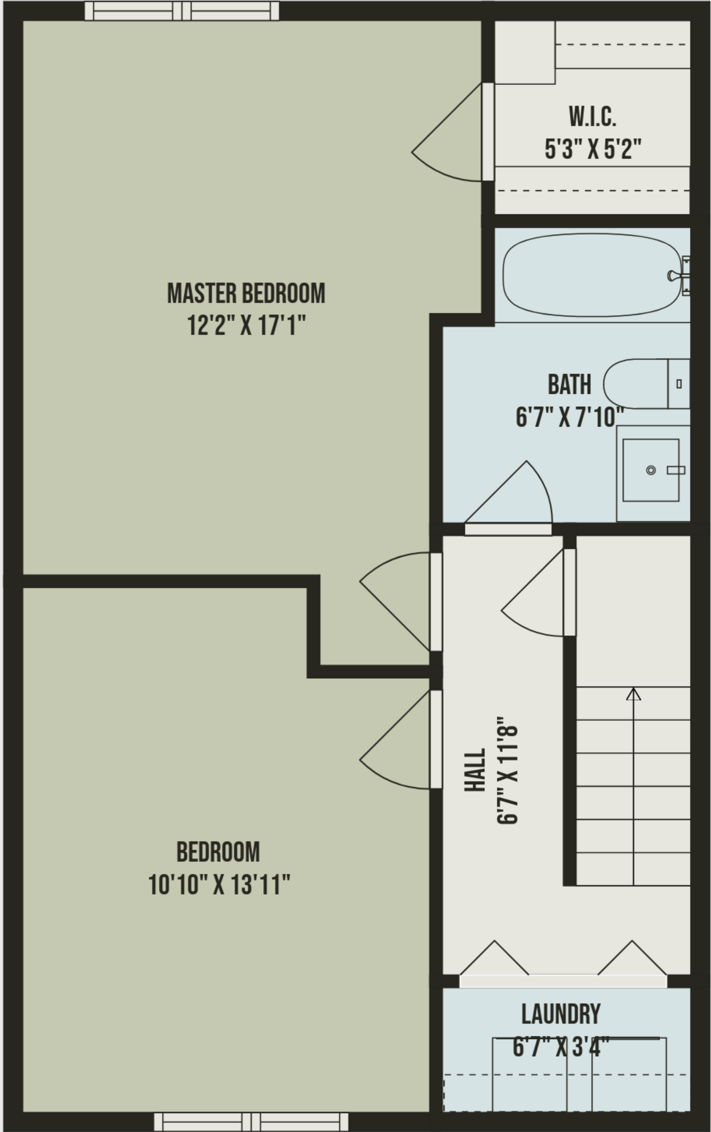
FLOOR 1
