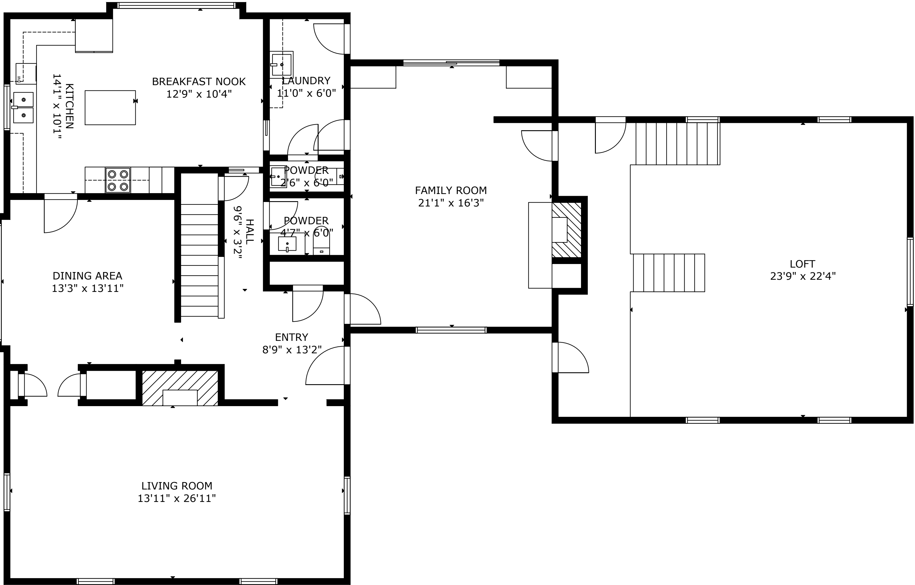
MAIN FLOOR GROSS INTERNAL AREA
