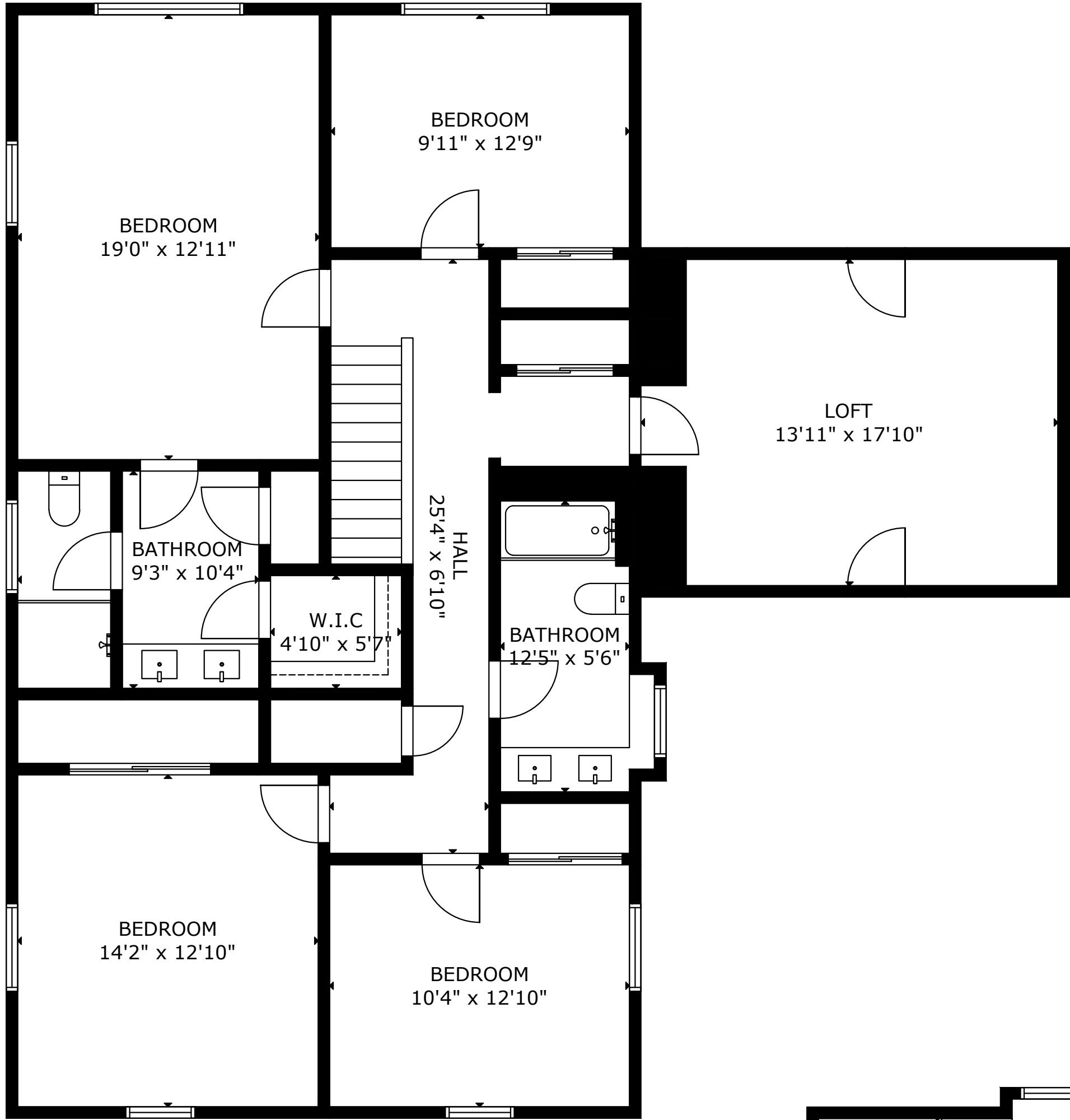
UPPER LEVEL 1
