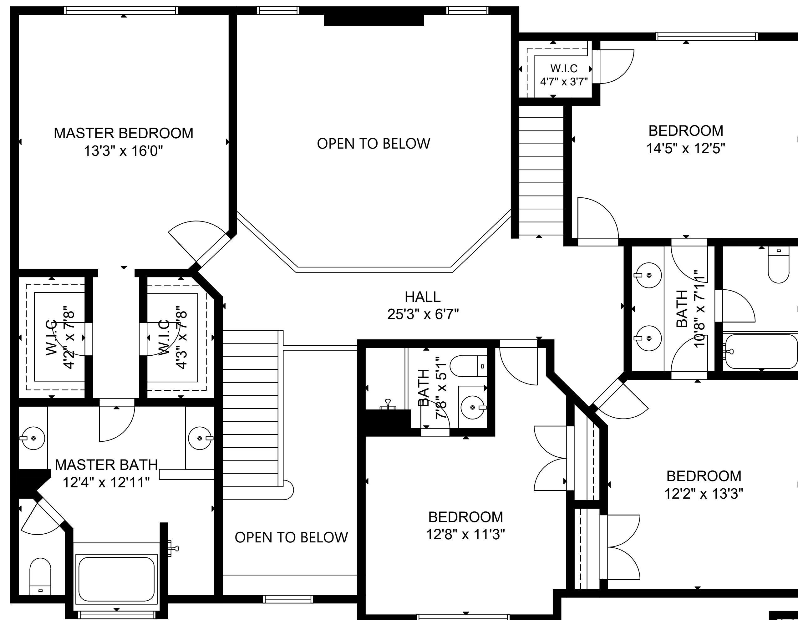
FLOOR 3
