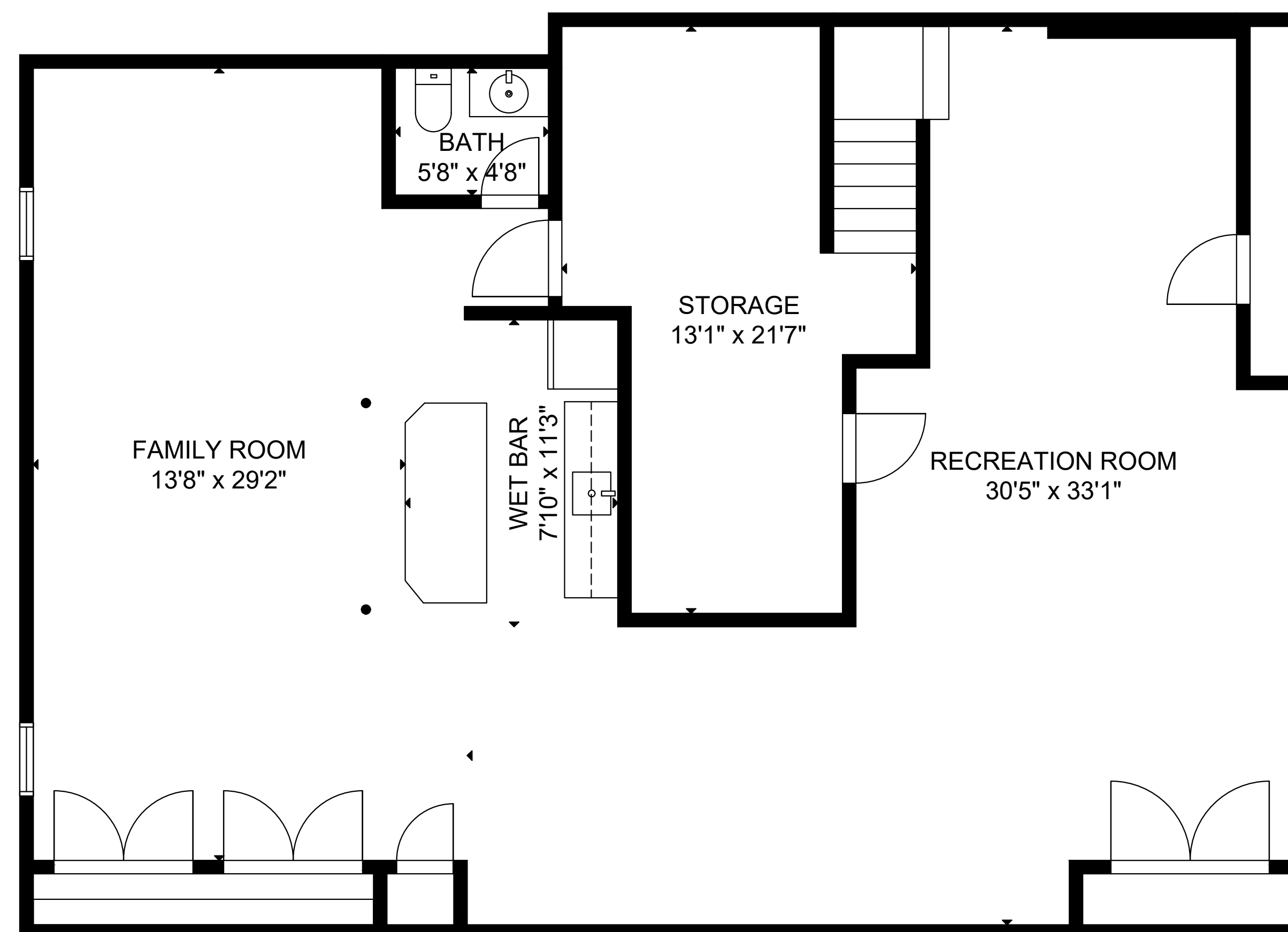
FLOOR 1
