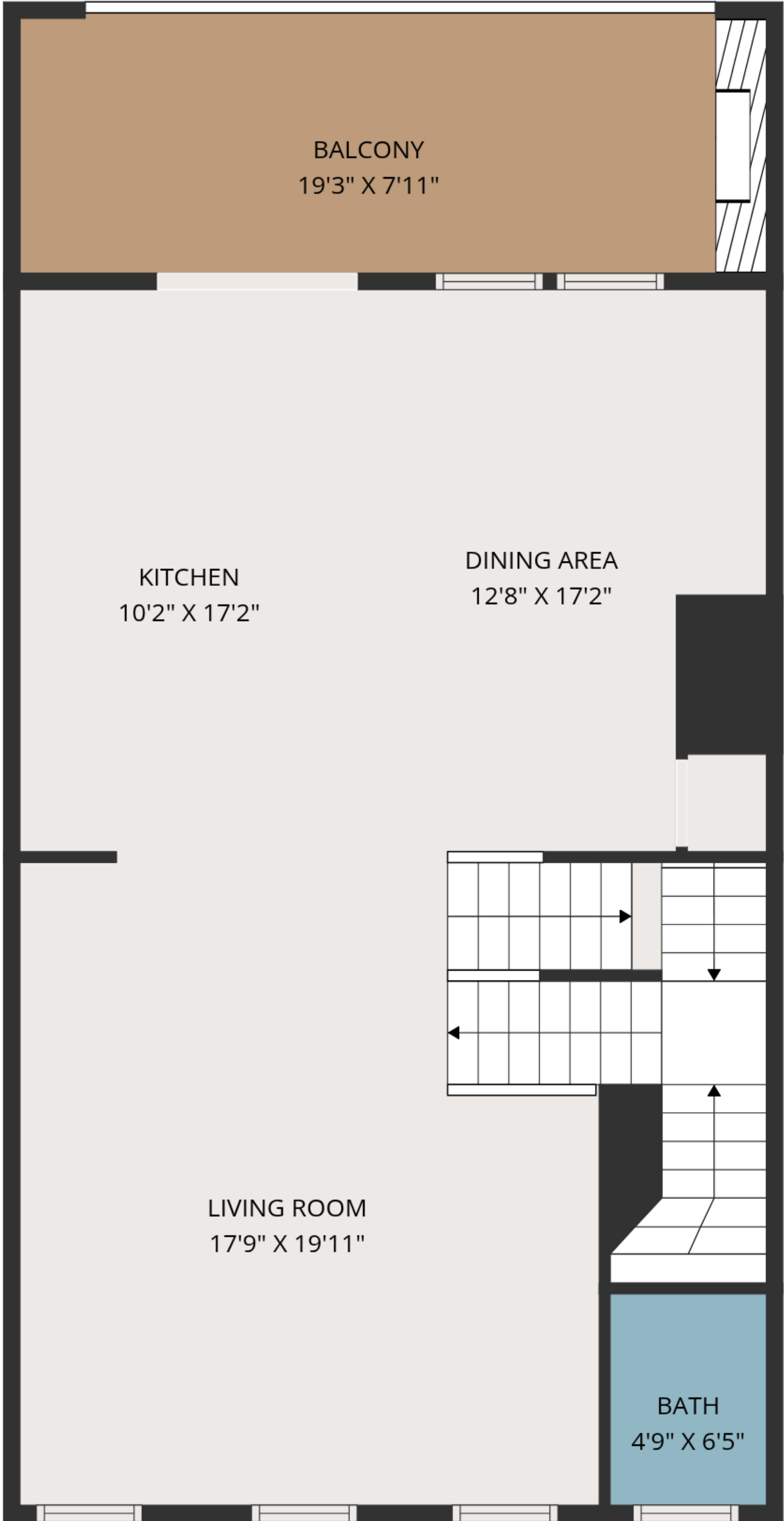
FLOOR 2
