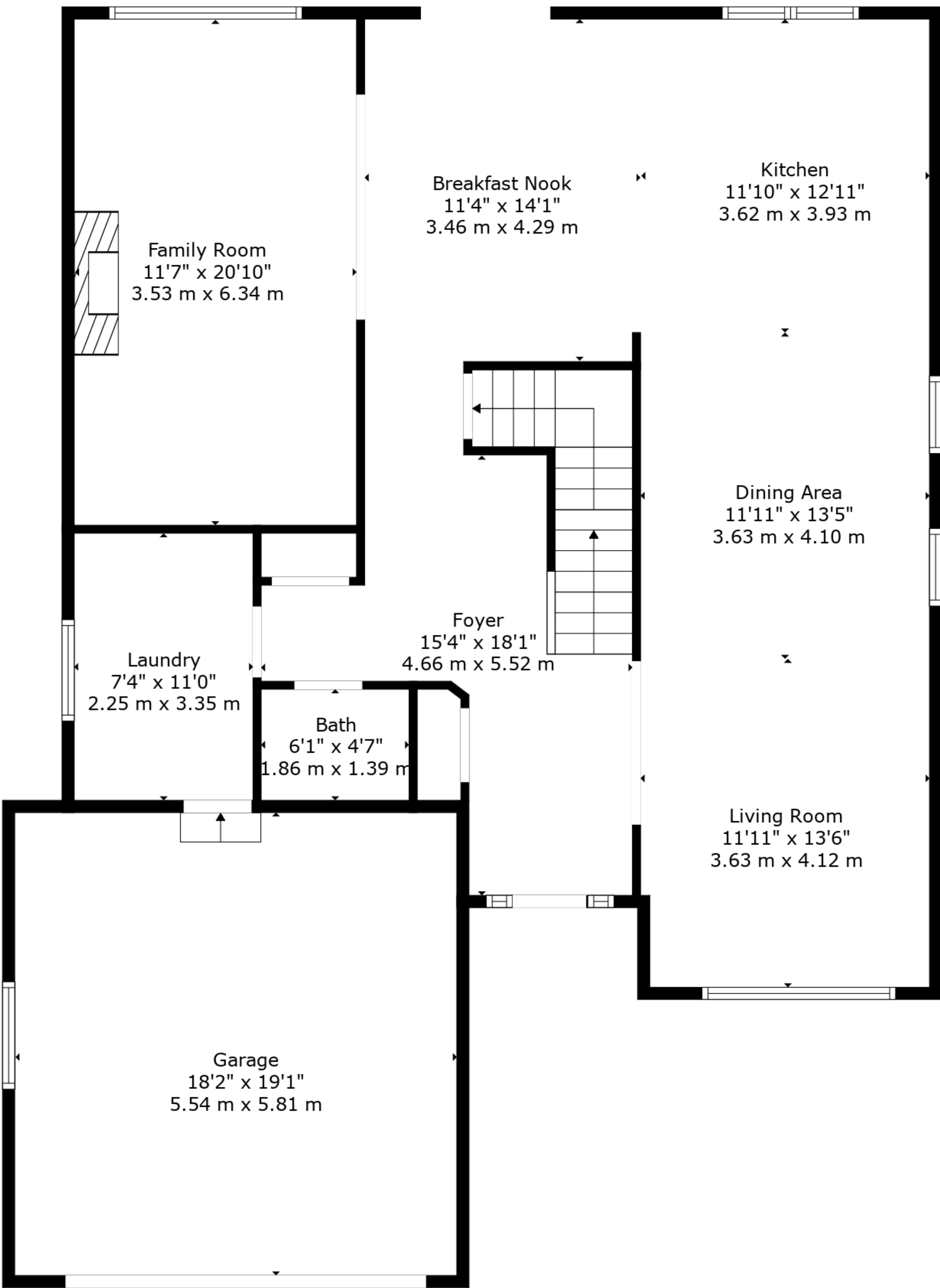
Floor 2
