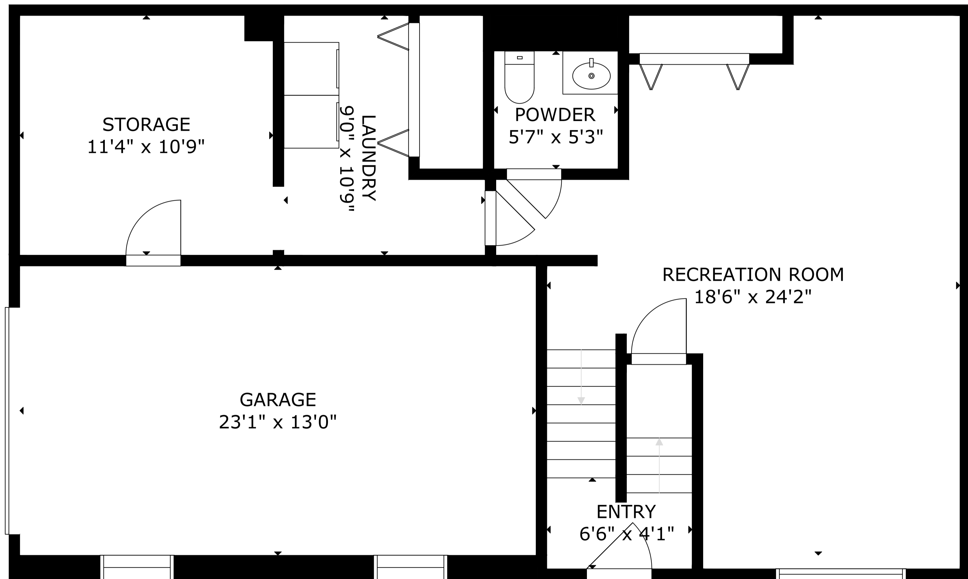
LOWER FLOOR
