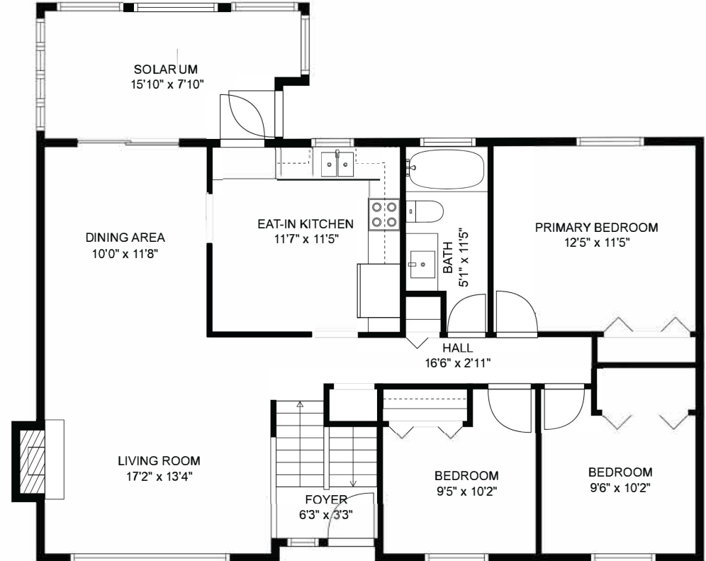
FLOOR 2
