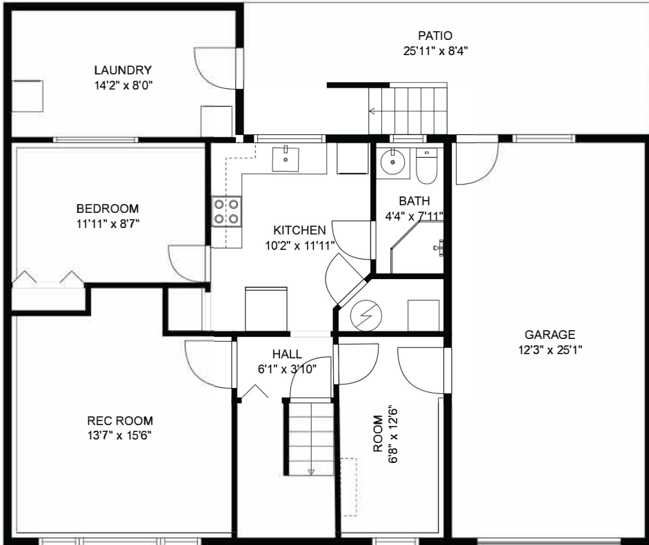
FLOOR 1
