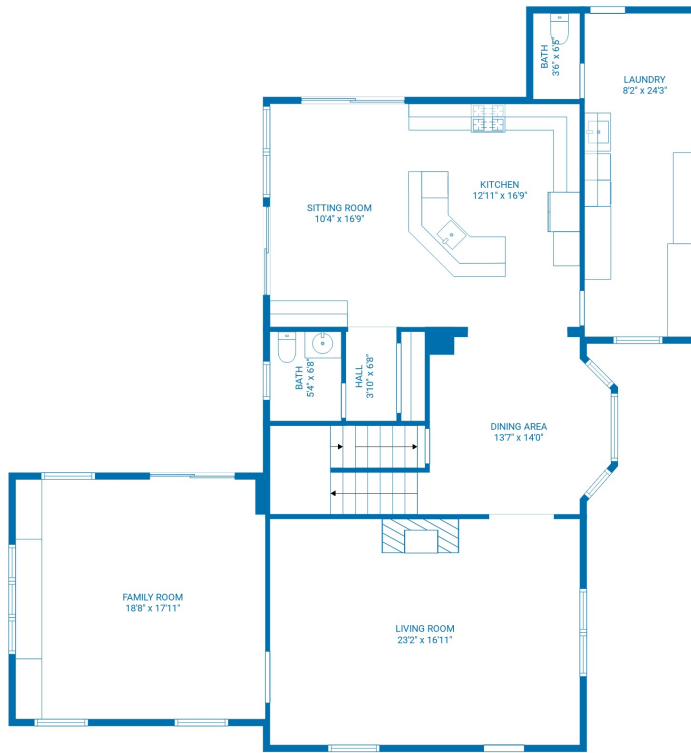
FLOOR 2
