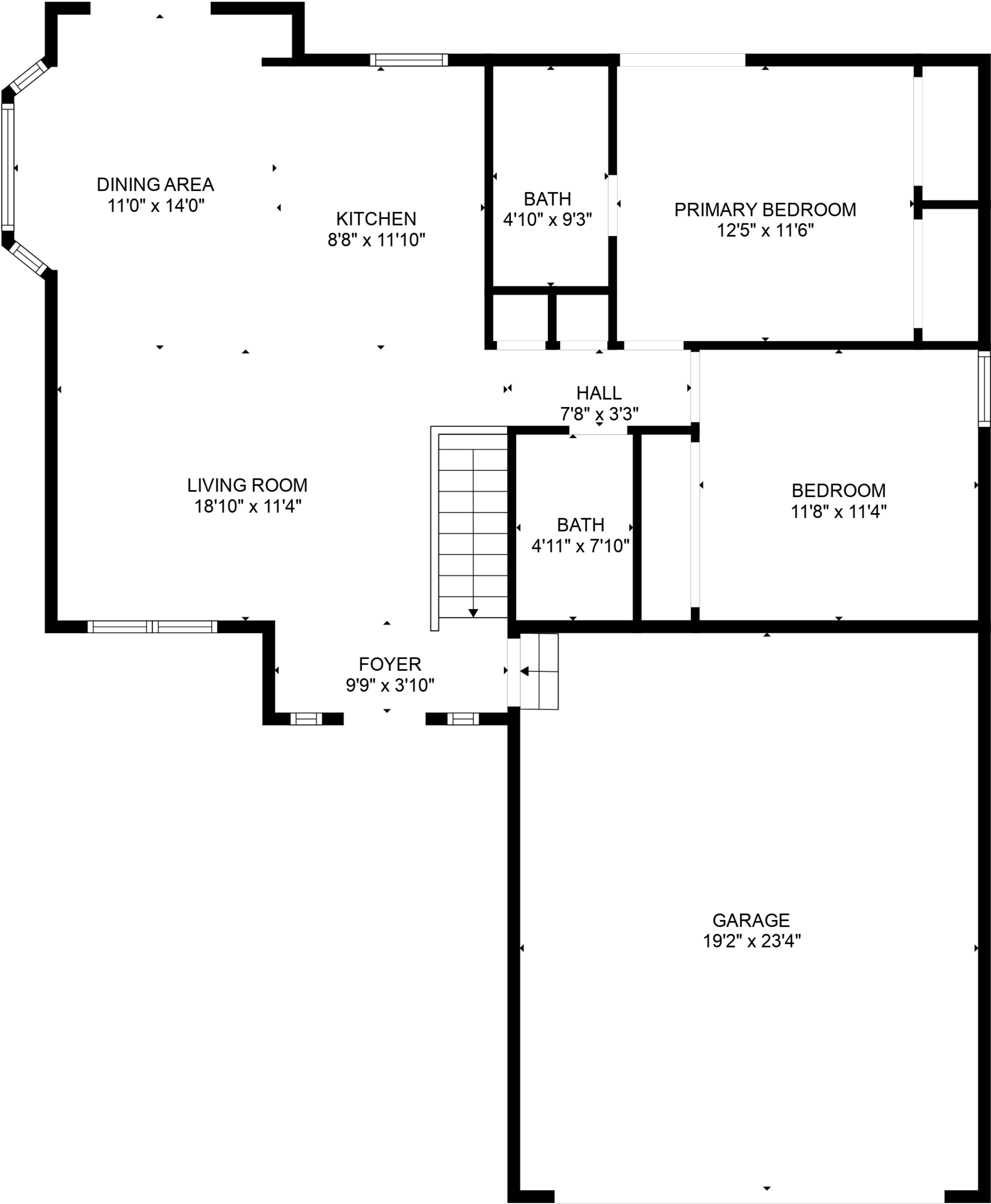
FLOOR 2
