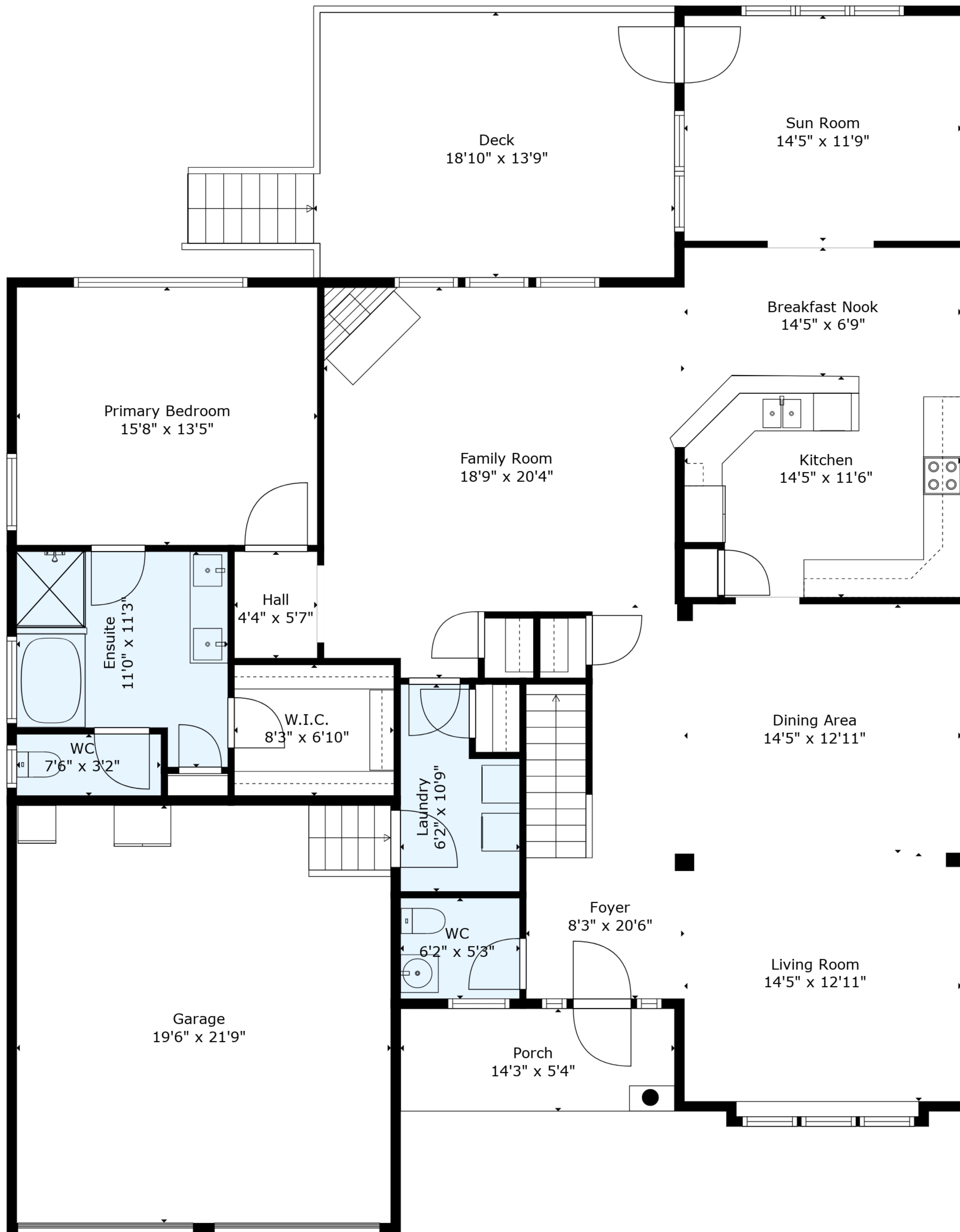
Floor 1
