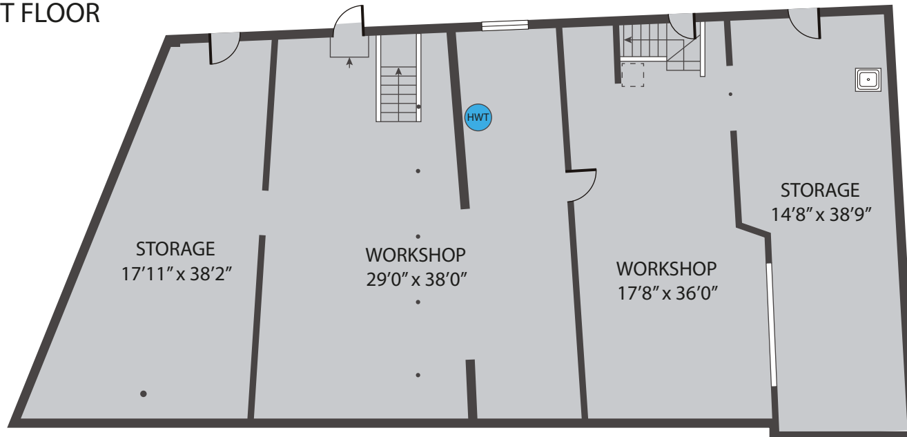
BASEMENT
