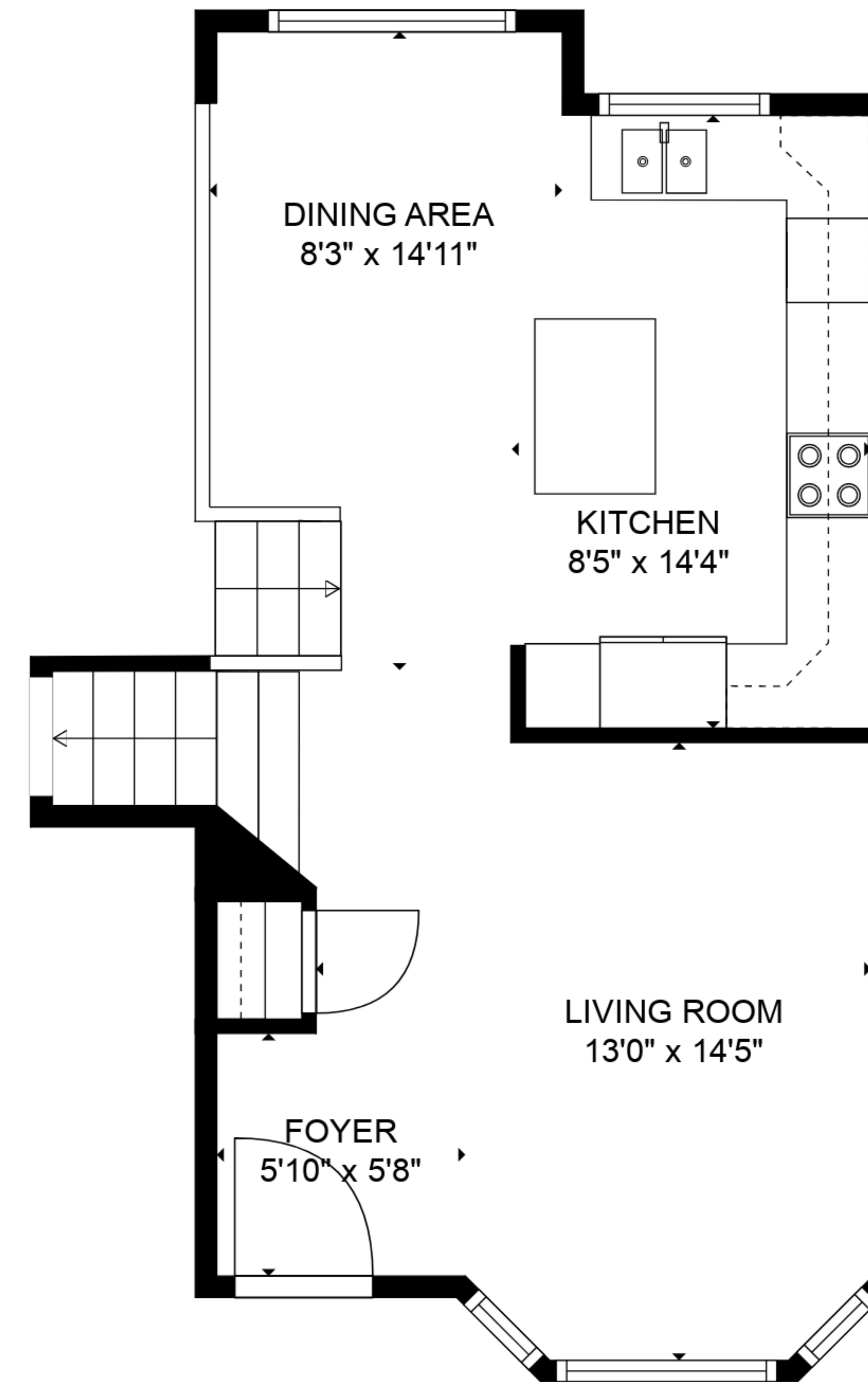
FLOOR 3
