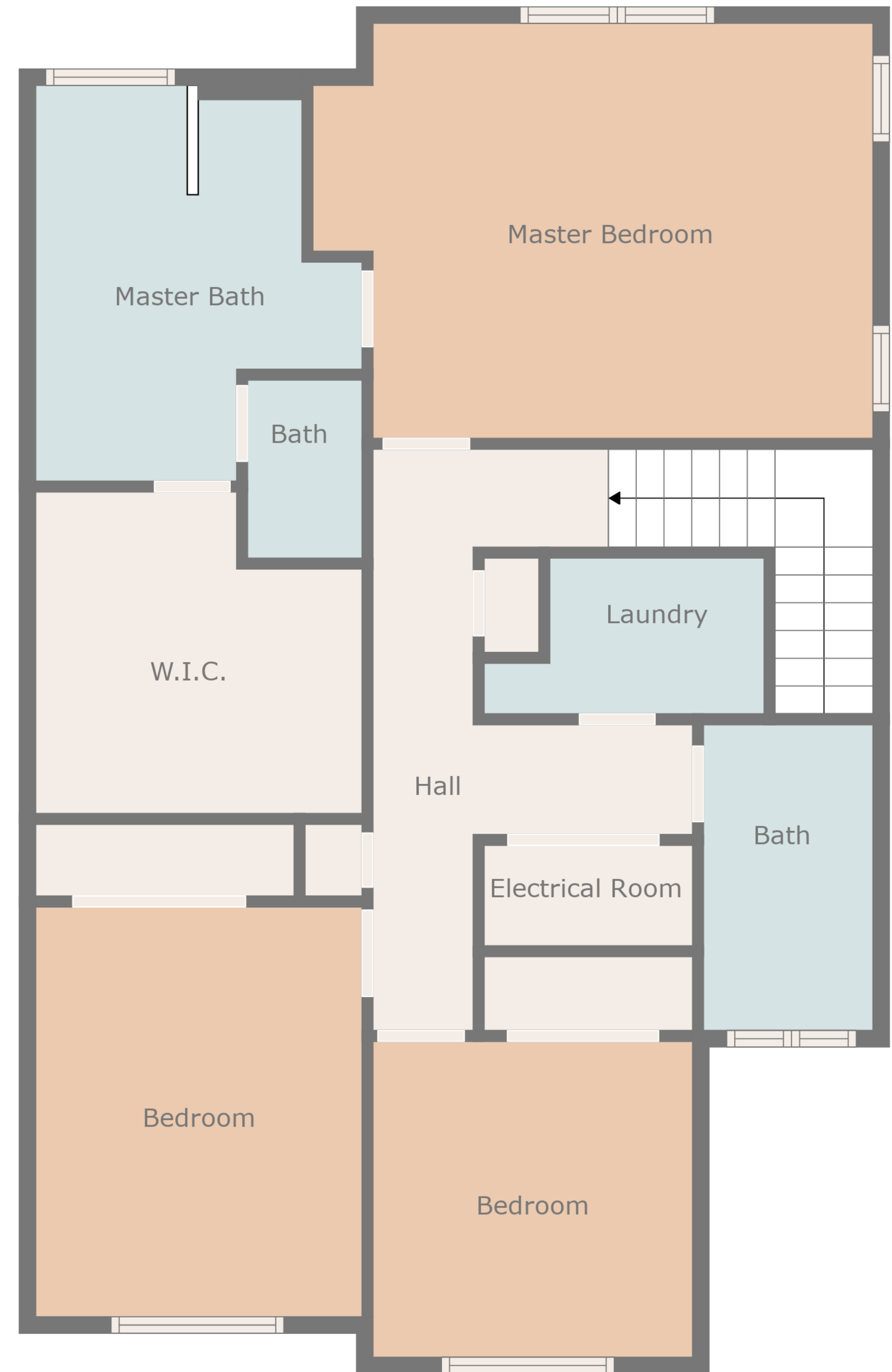
Floor 2
