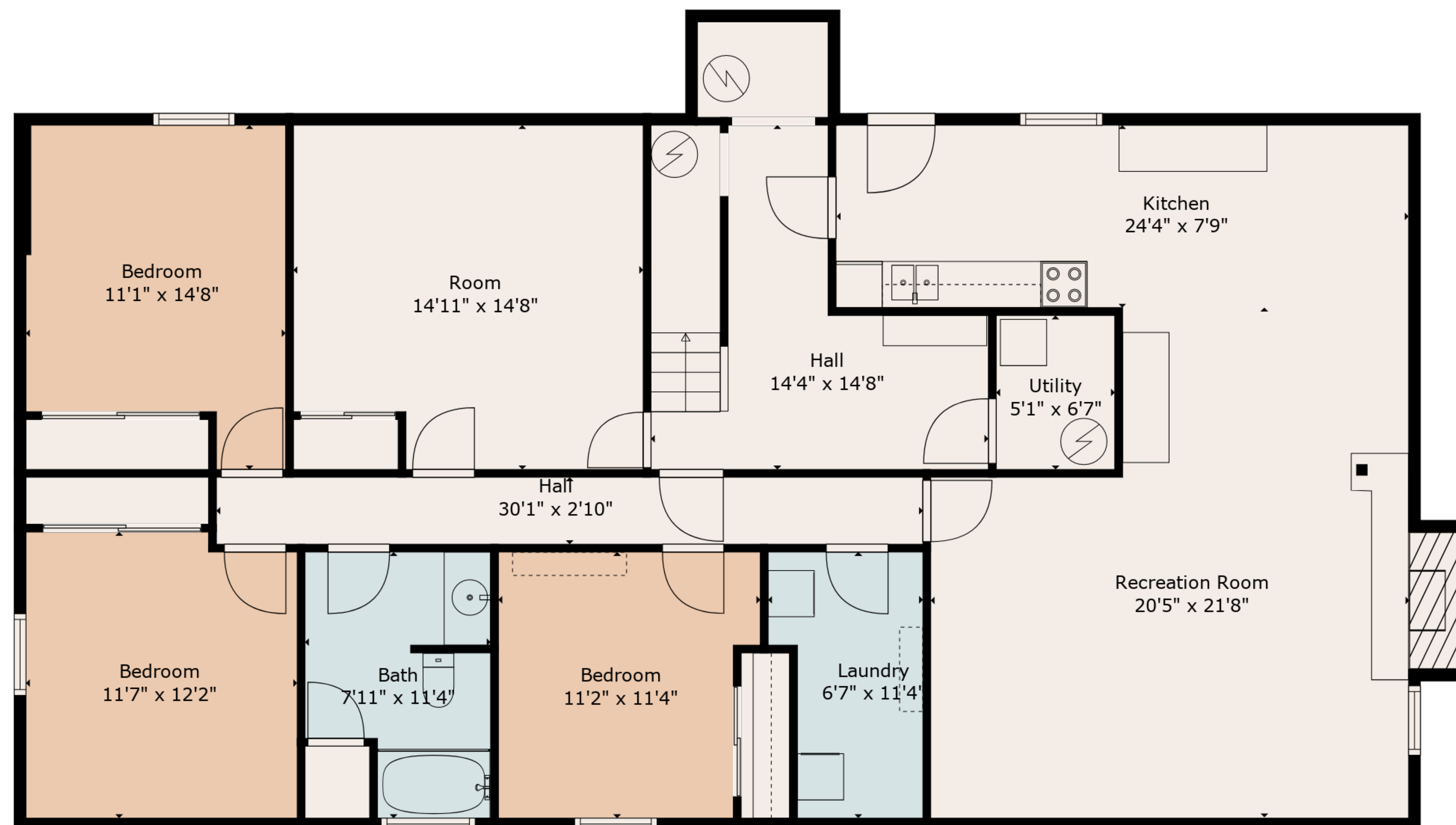
Floor 2
