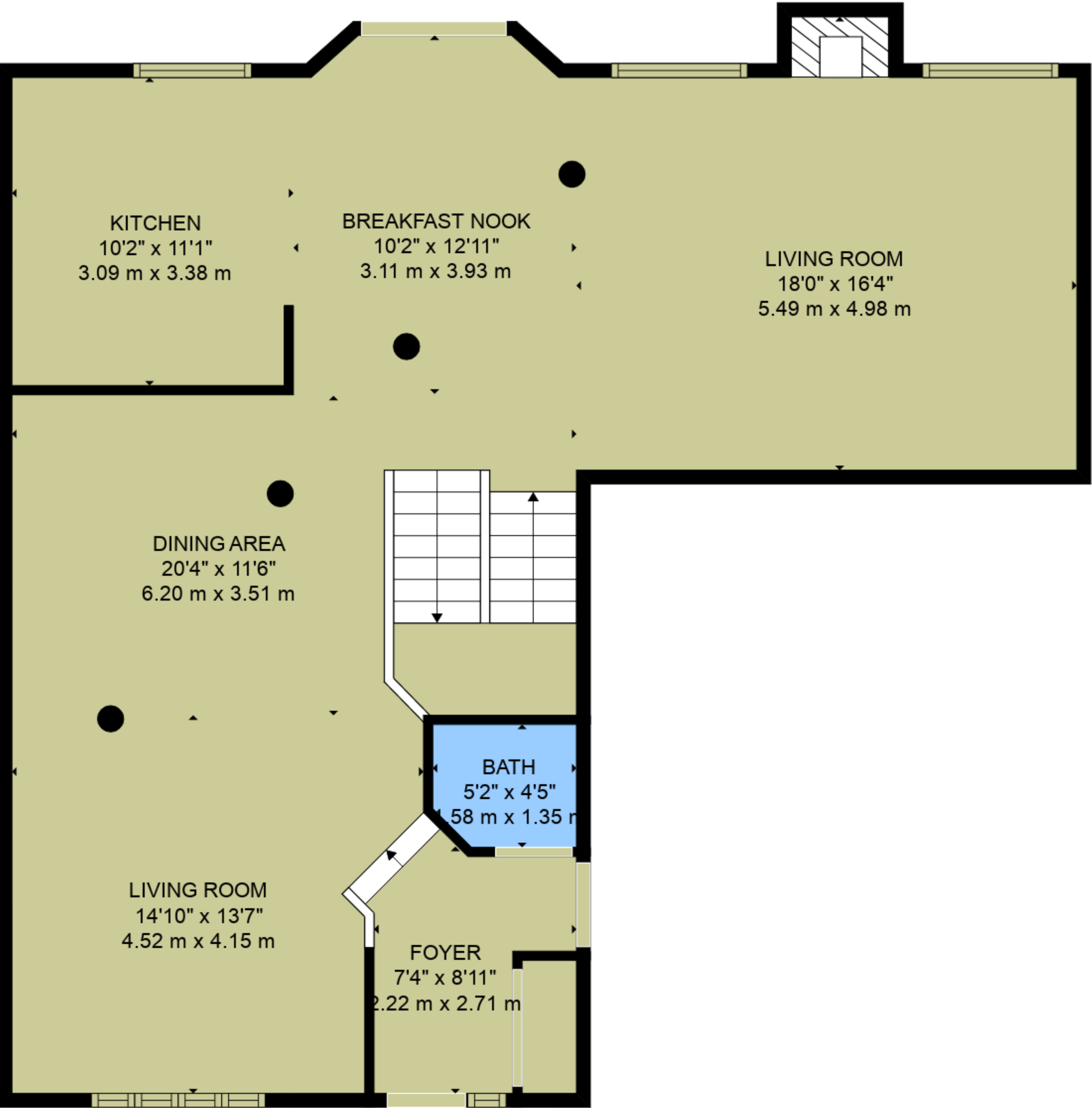
FLOOR 2
