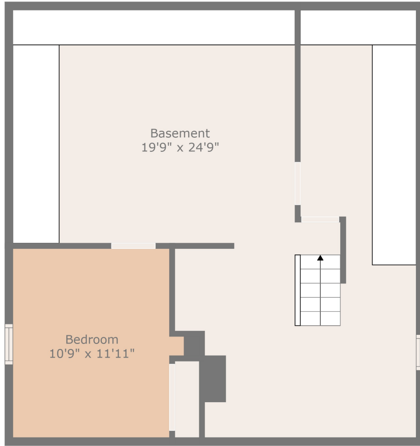
Floor 1
