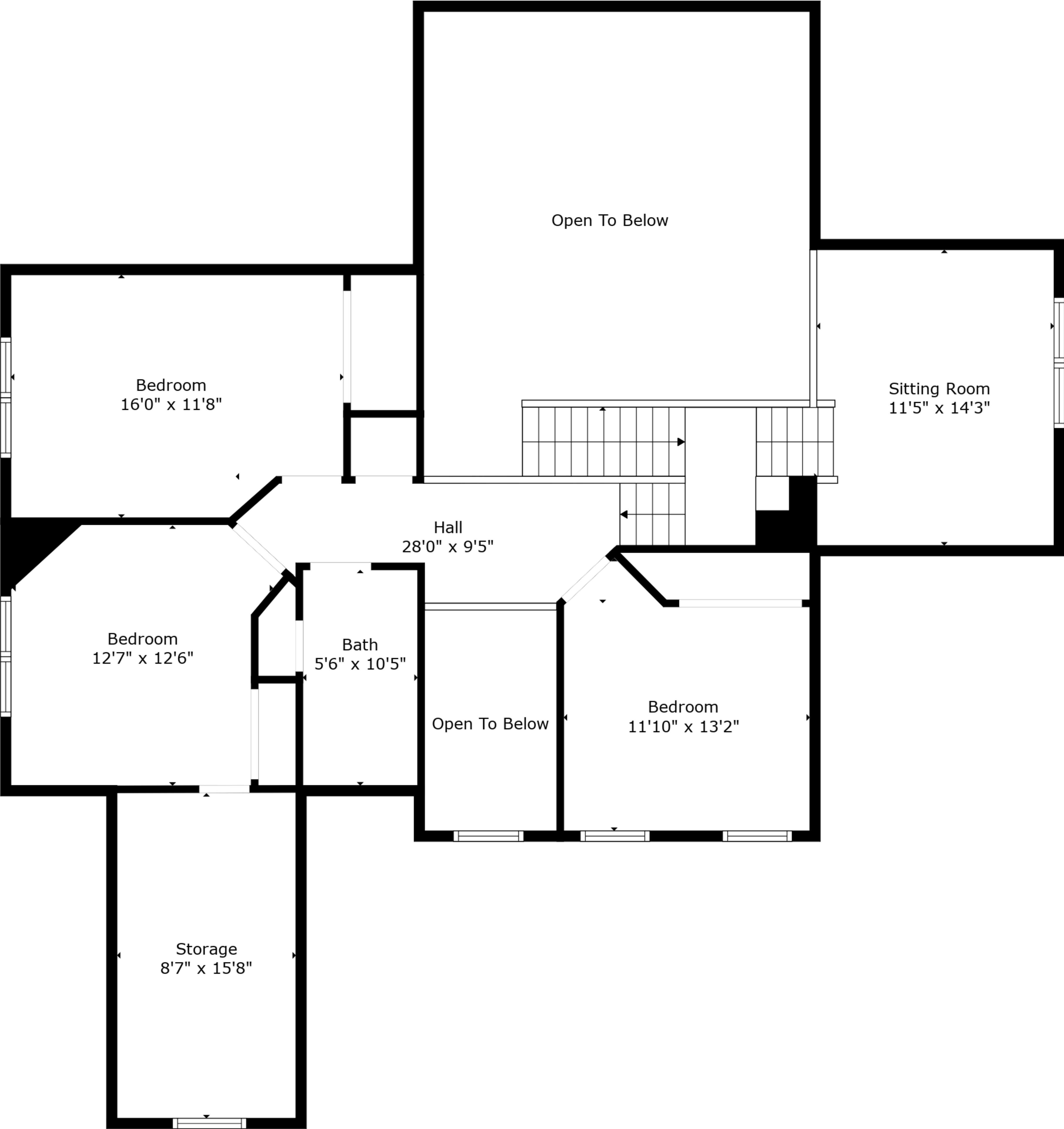
Floor 2
