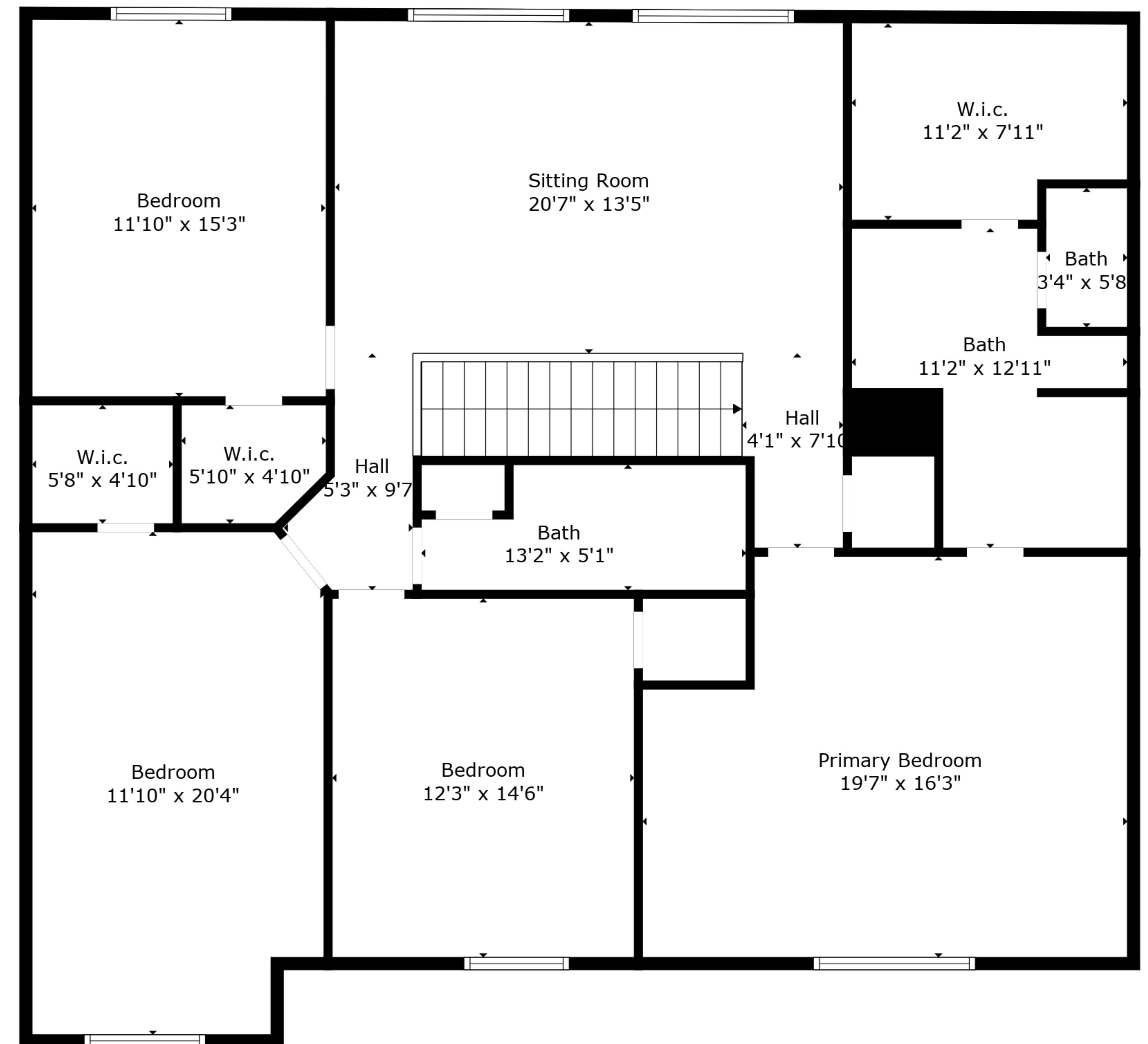
Floor 2
