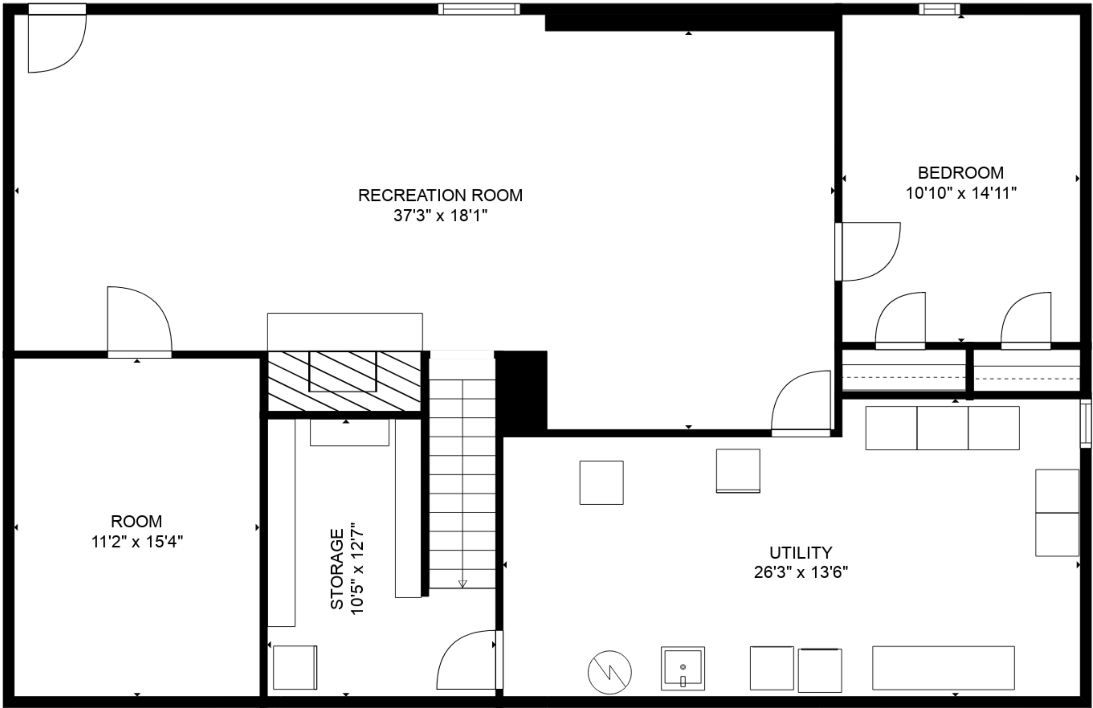
FLOOR 1
