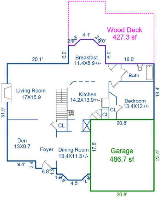
First Floor 1419.1 sf
