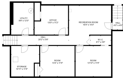
FLOOR 1
