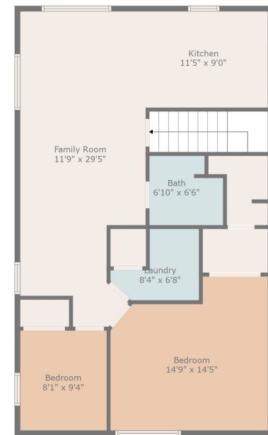
Floor 2
