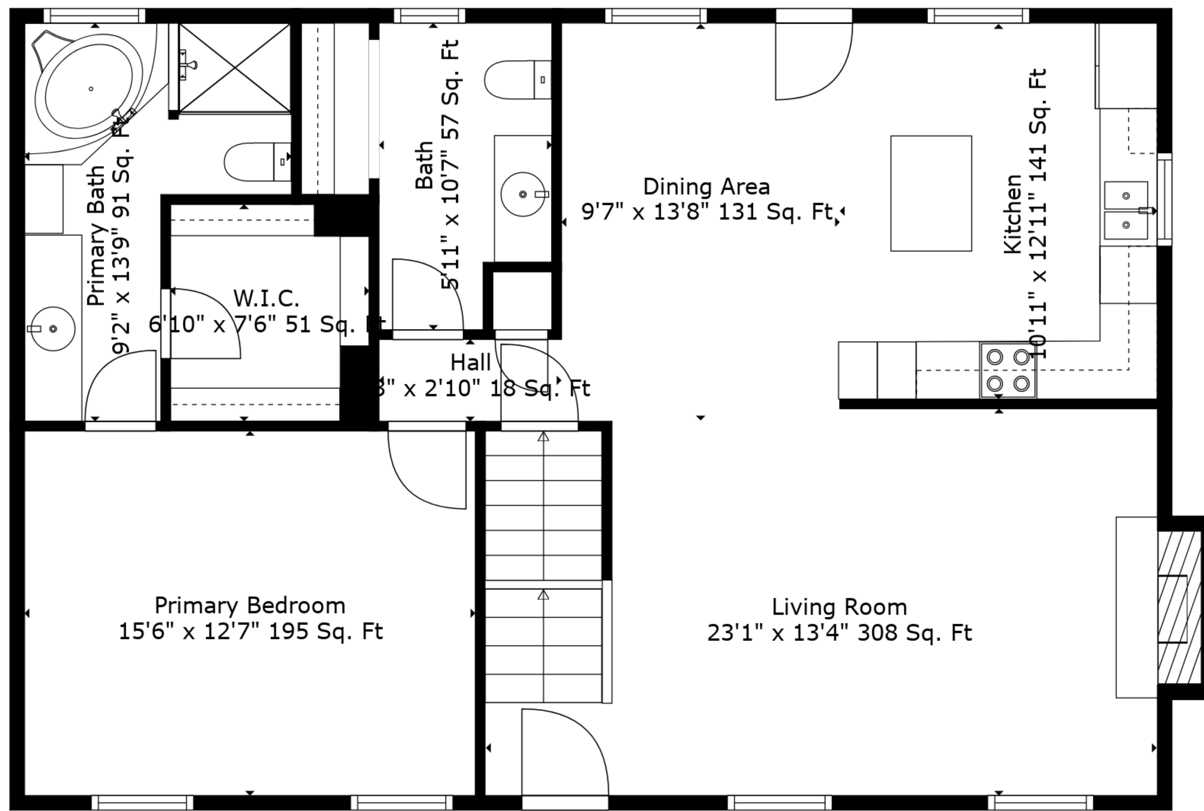
Floor 2
