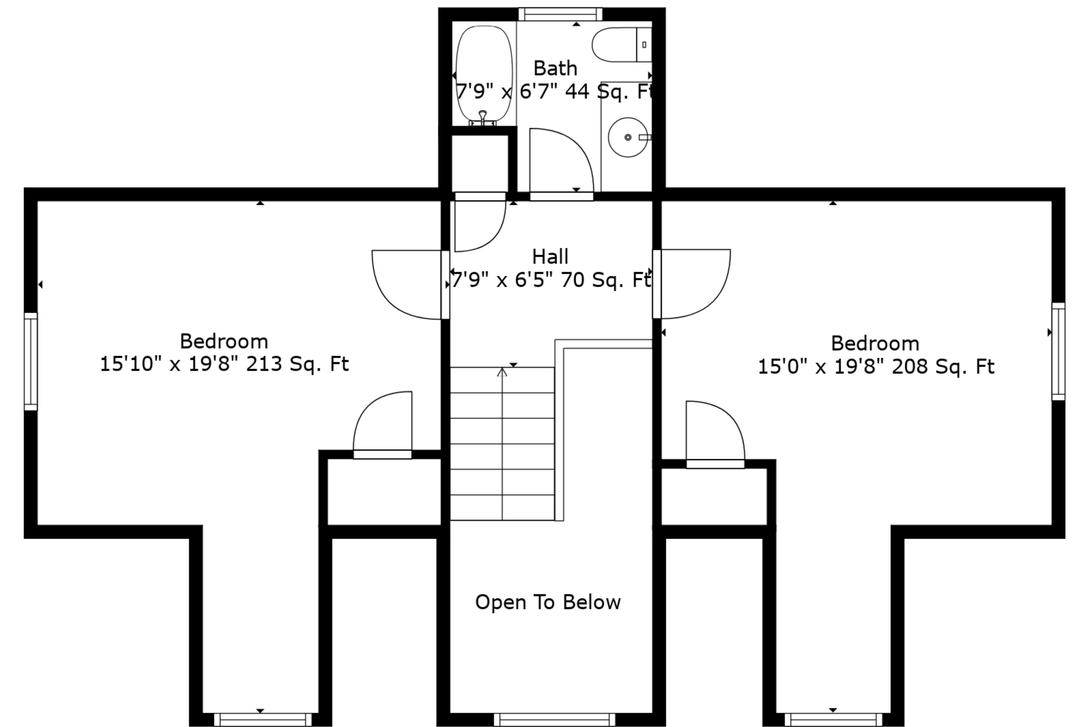
Floor 3
