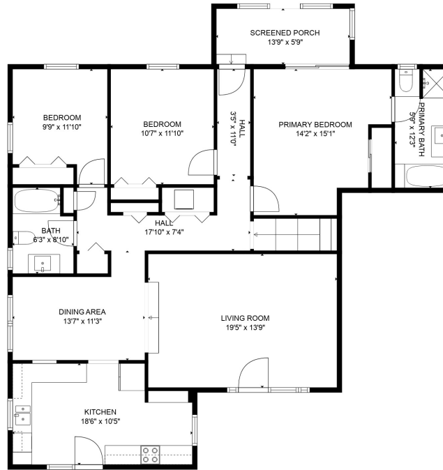
FLOOR 2
