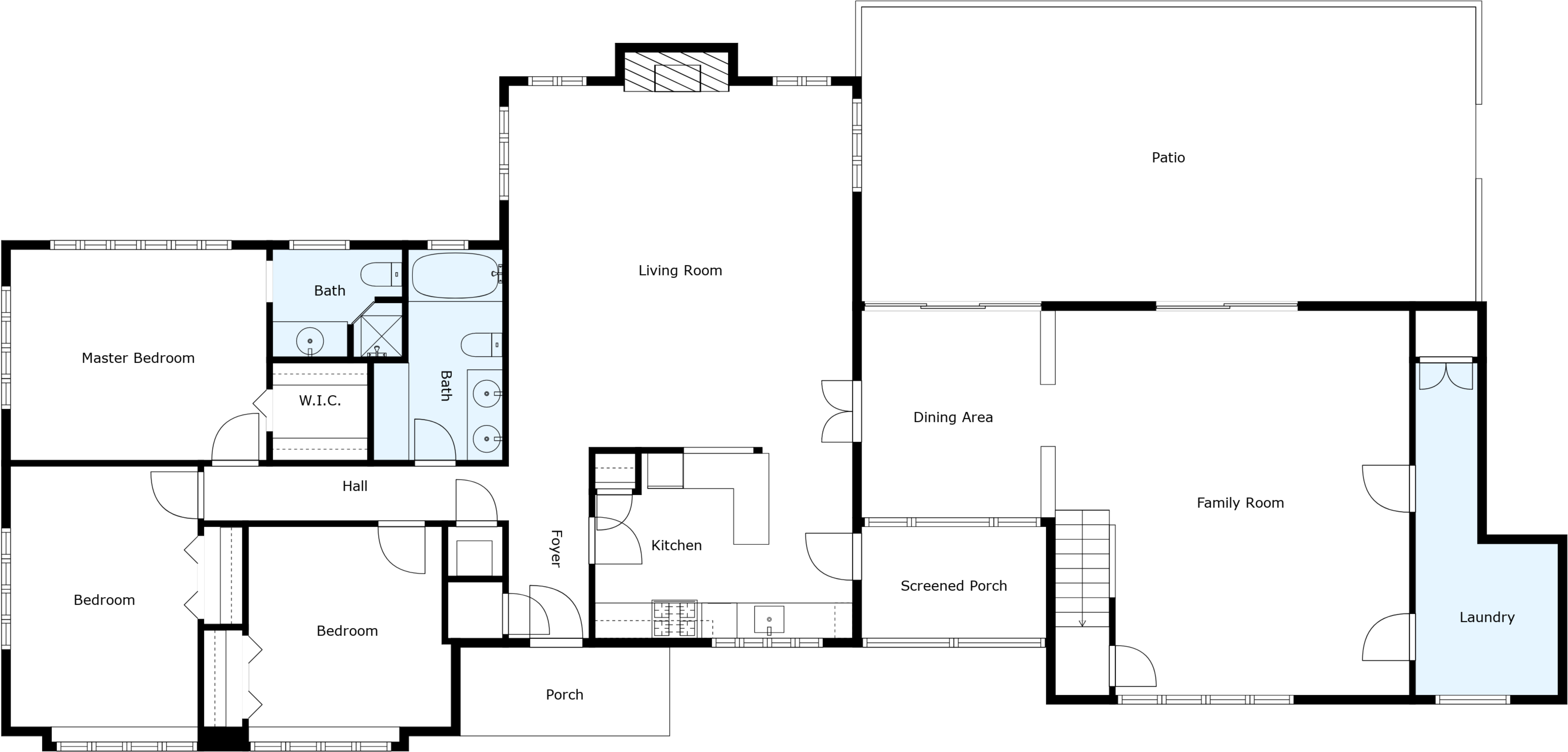
Floor 1
