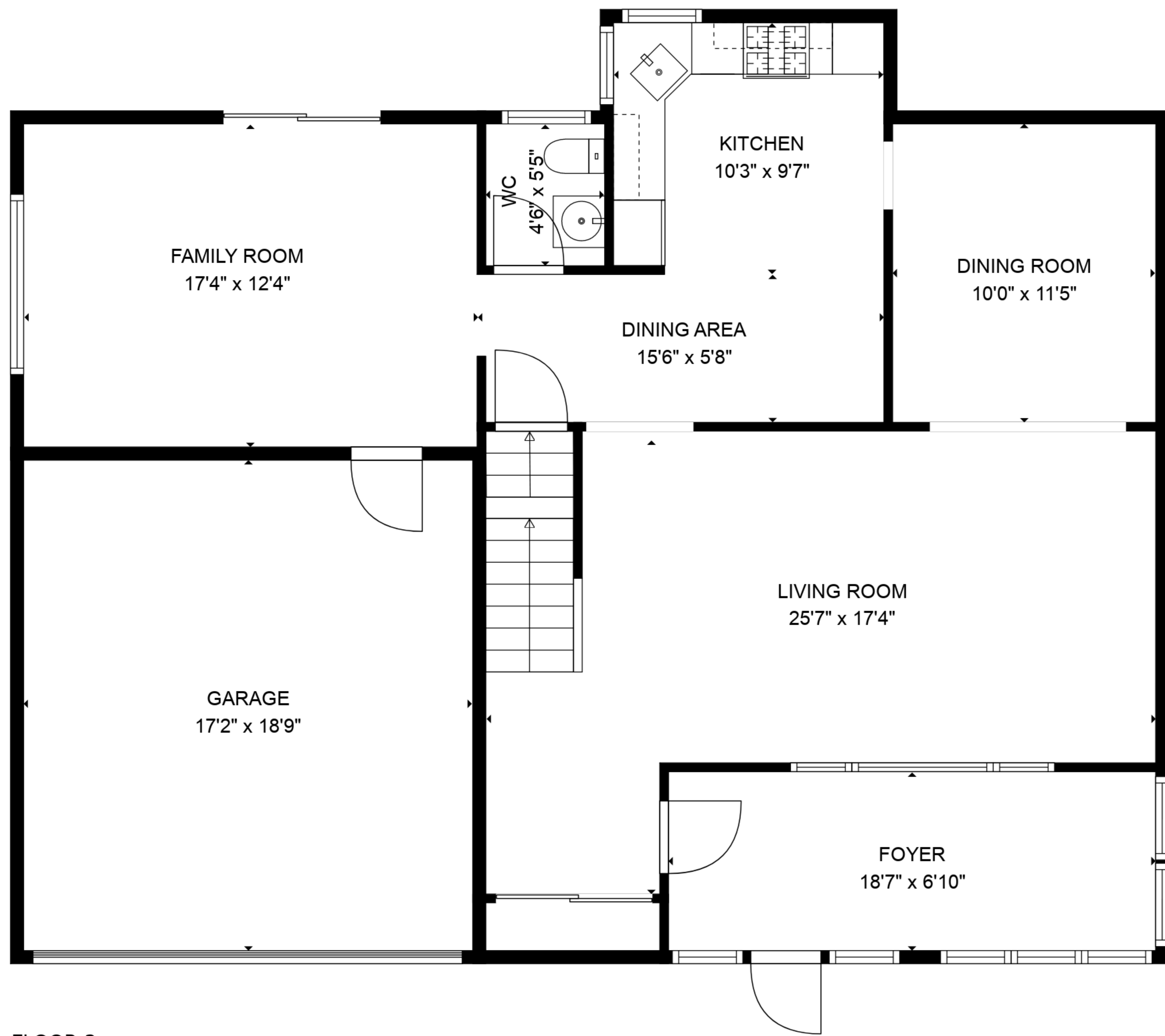
FLOOR 2
