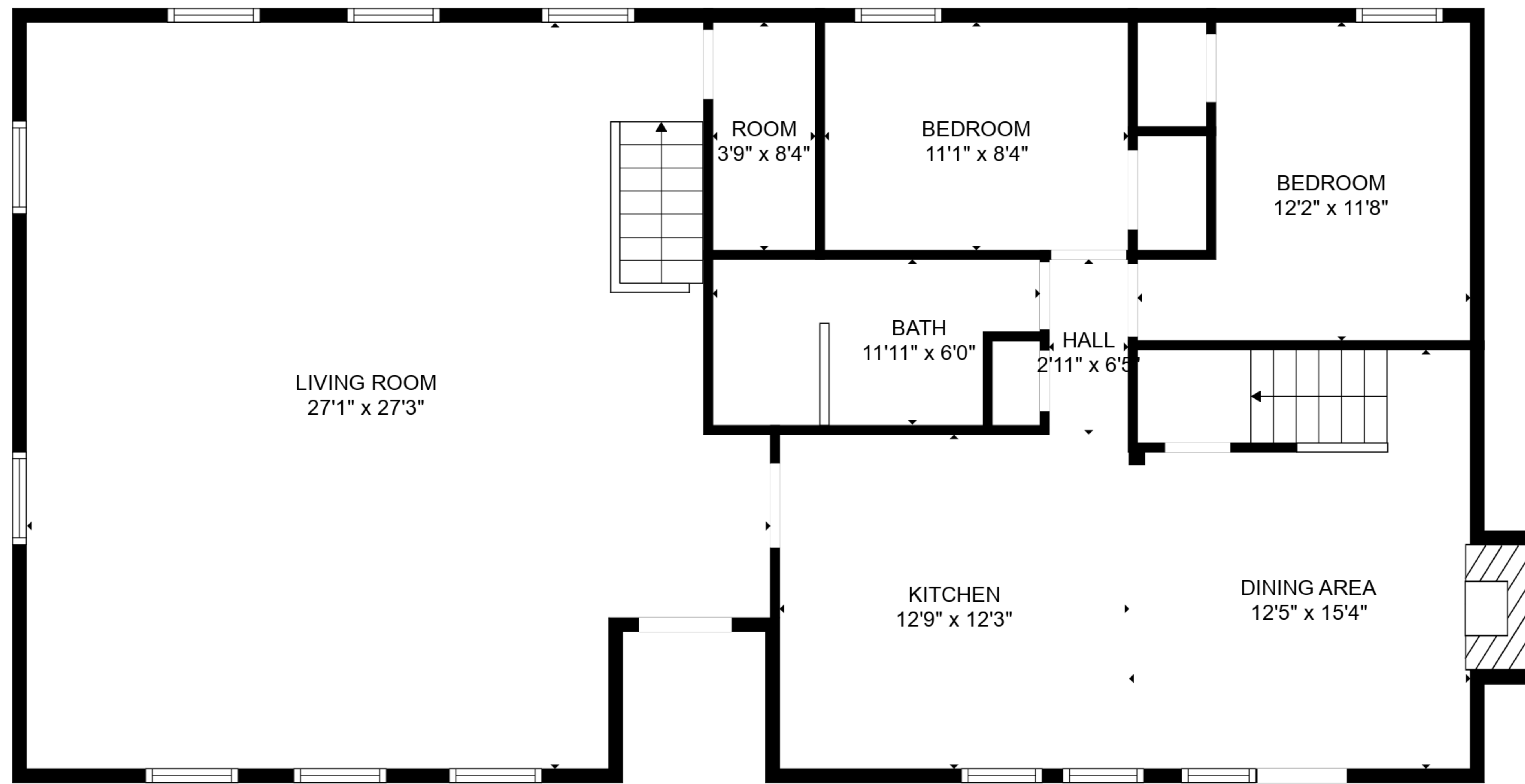
FLOOR 2
