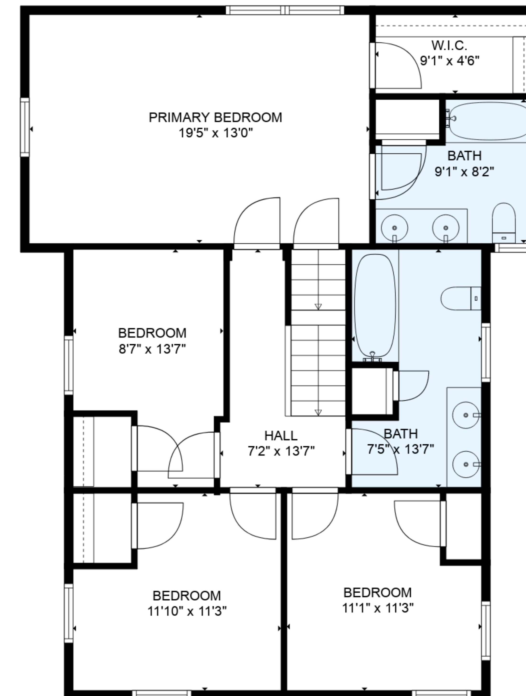
FLOOR 2
