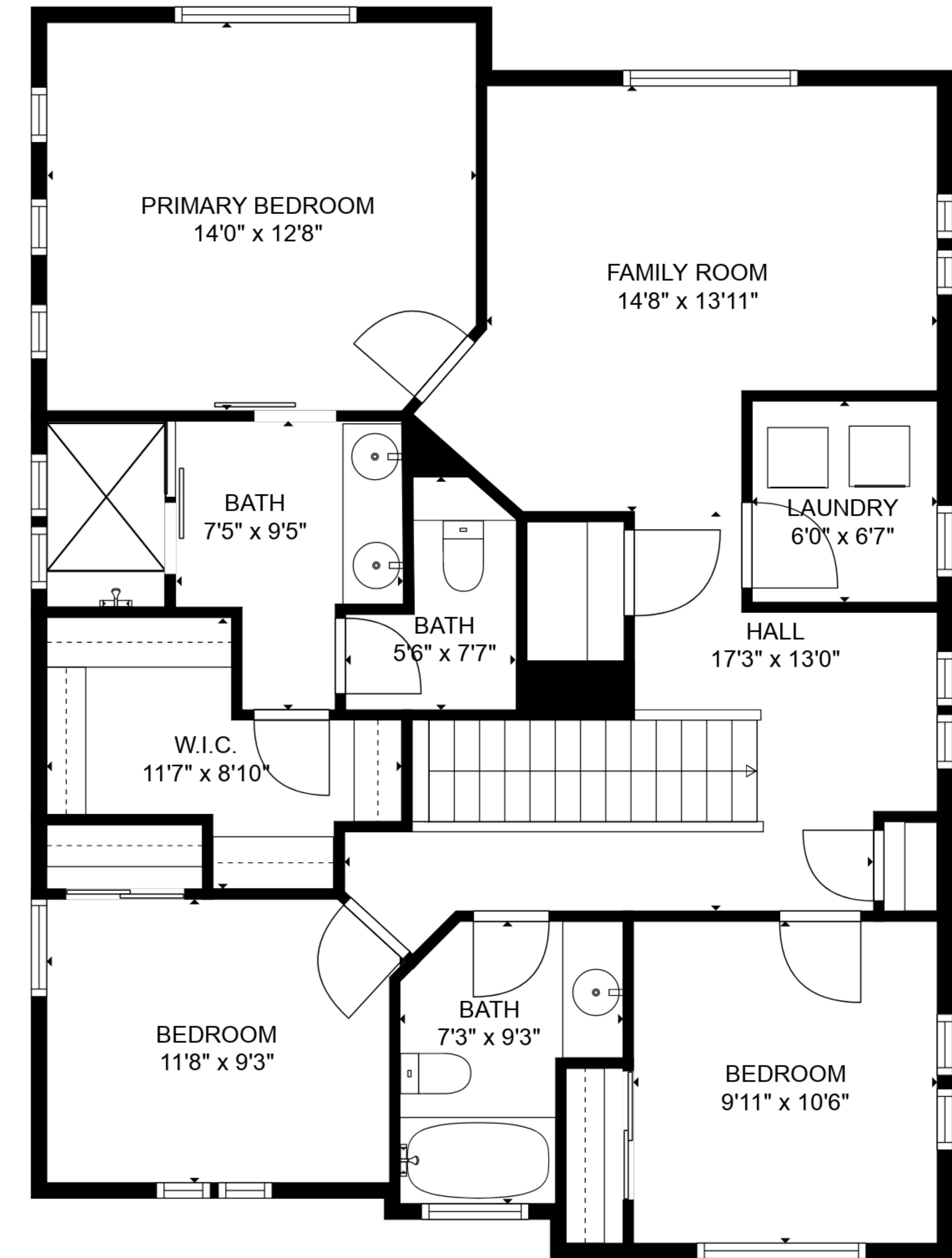
FLOOR 3
