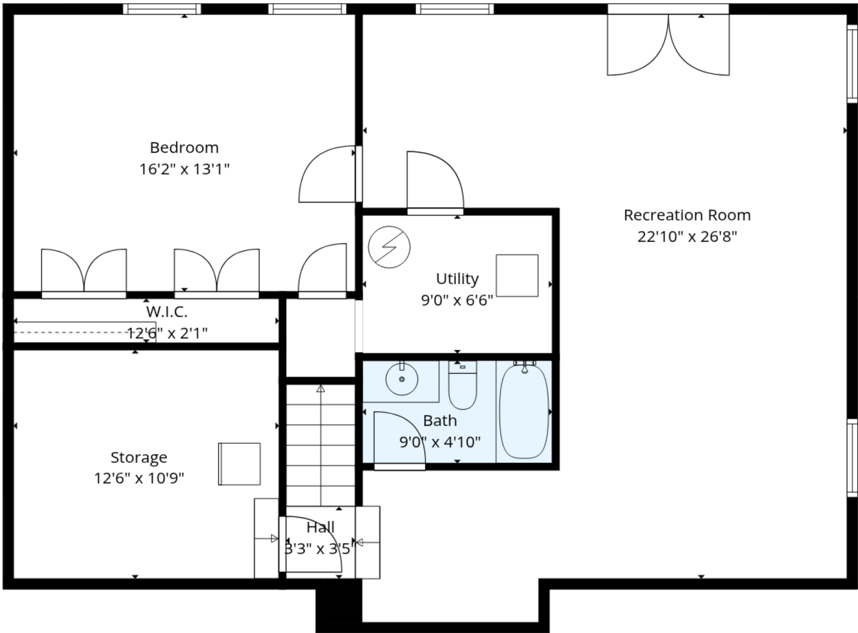
Floor 1
