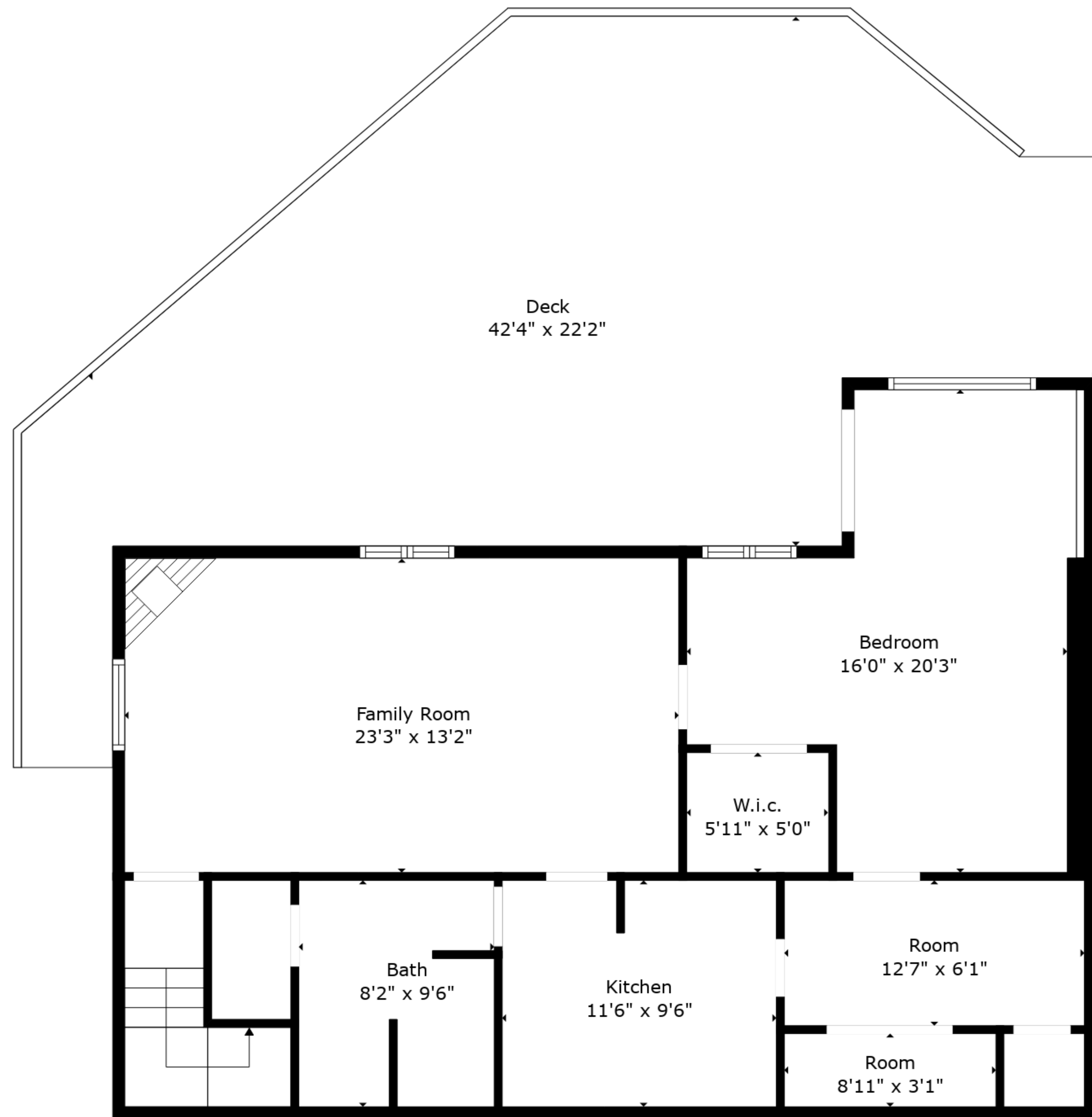
Floor 1
