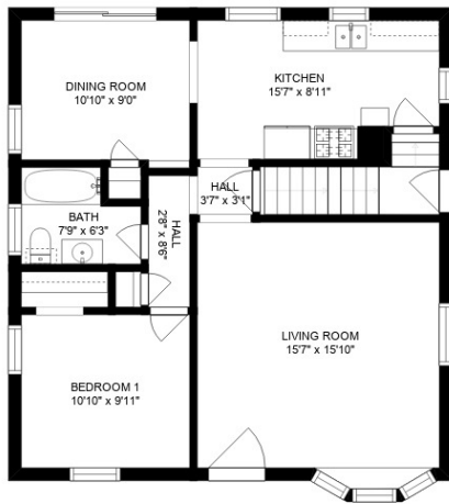
MAIN FLOOR
