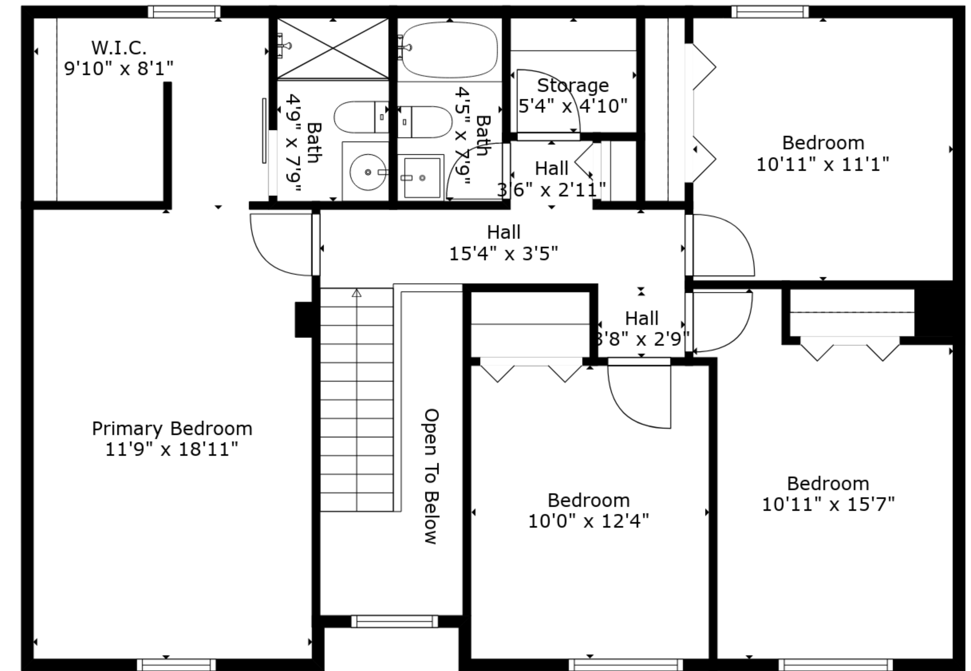
Floor 3
