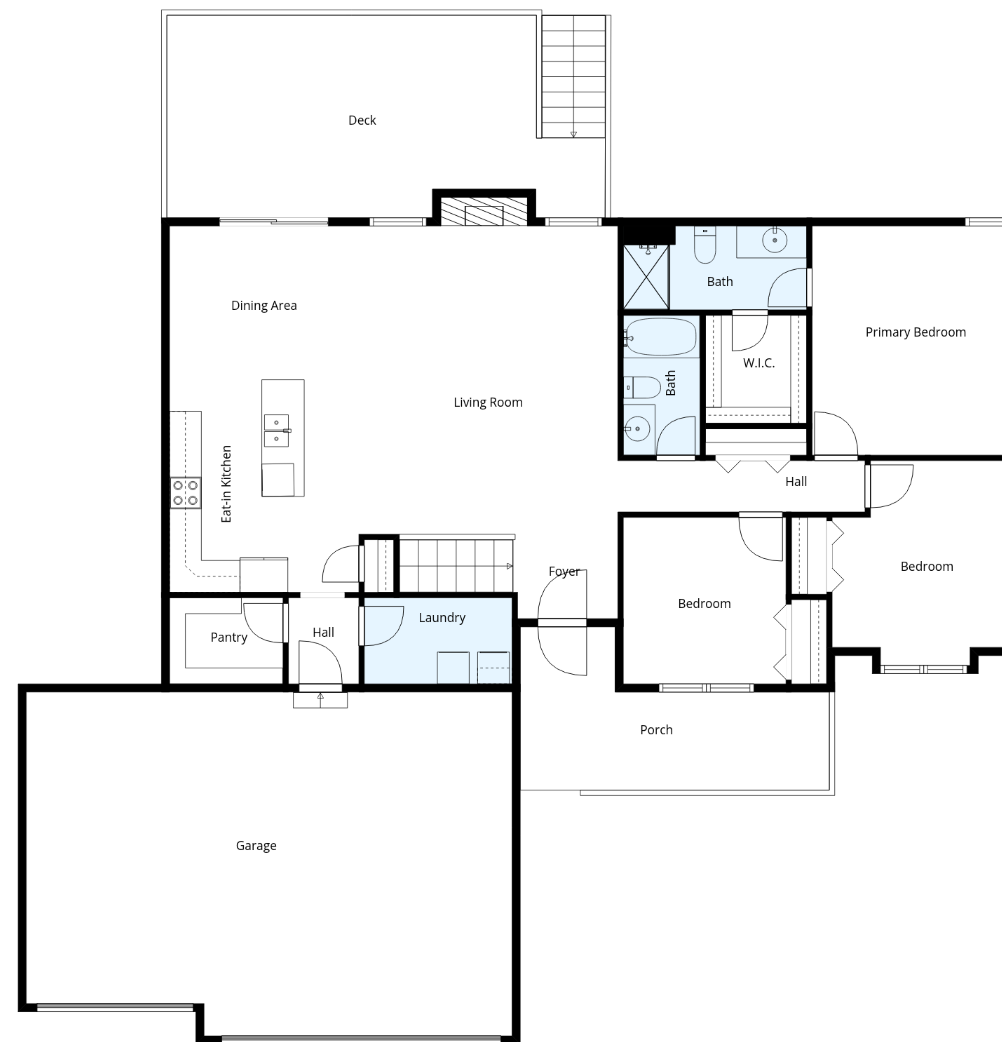
Floor 2
