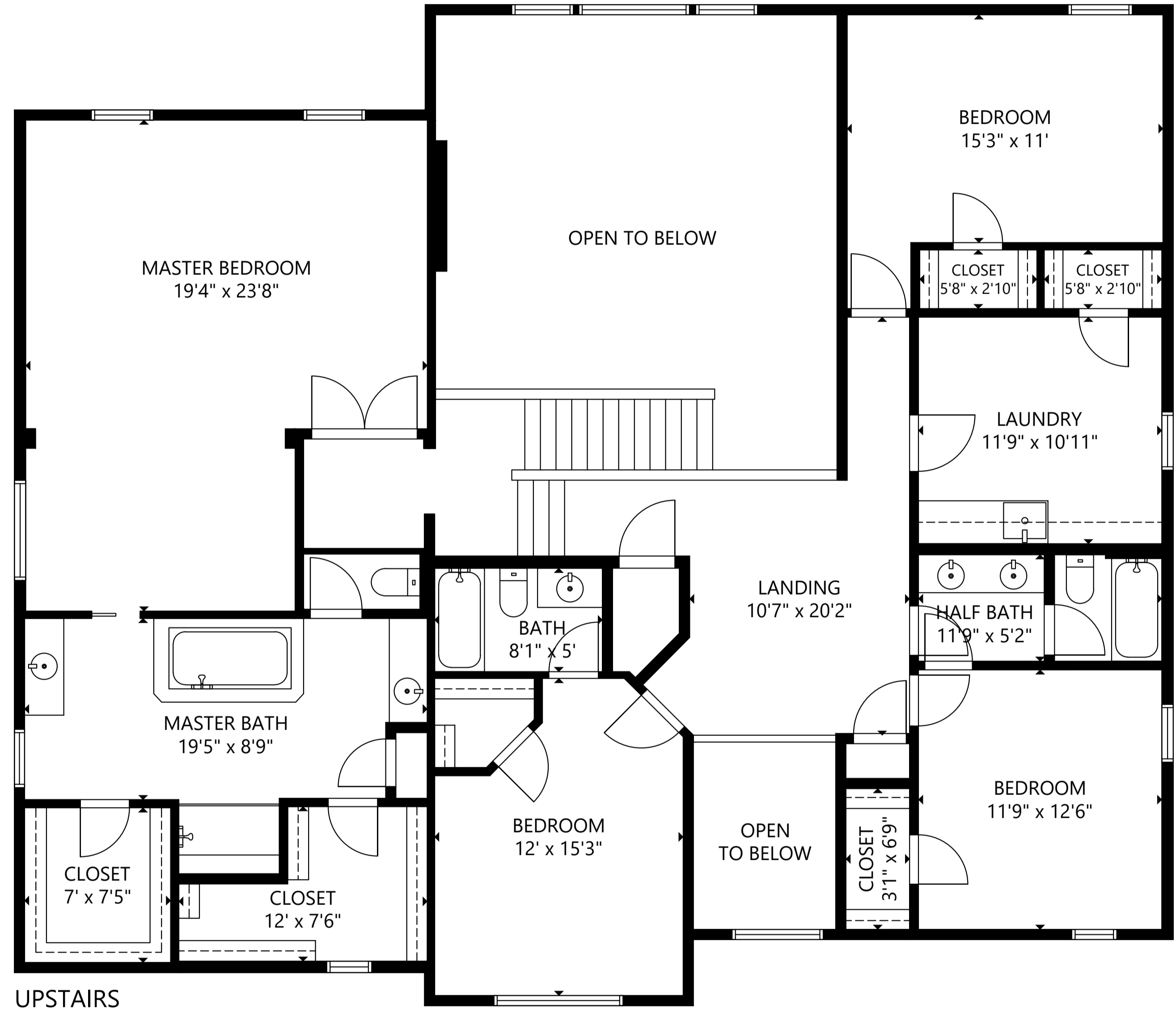
UPSTAIRS
