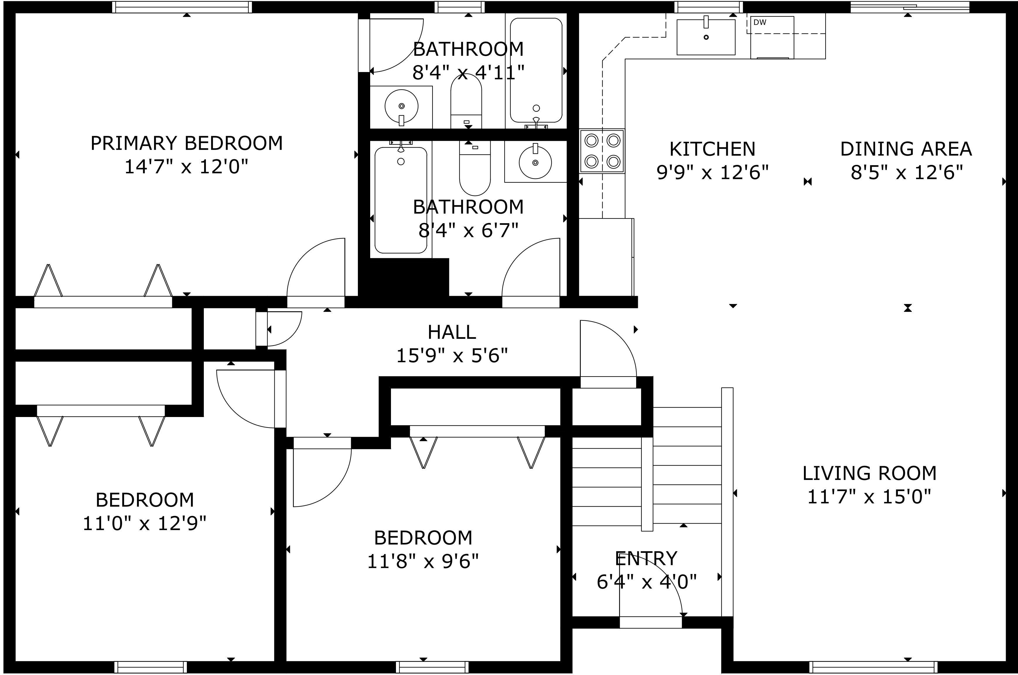
MAIN FLOOR
