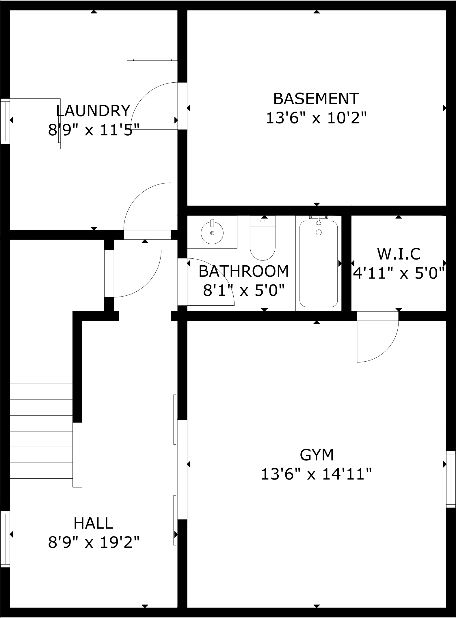
LOWER FLOOR
