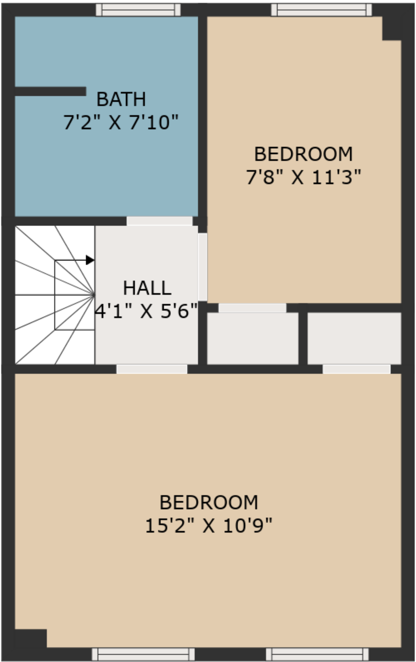
FLOOR 3
