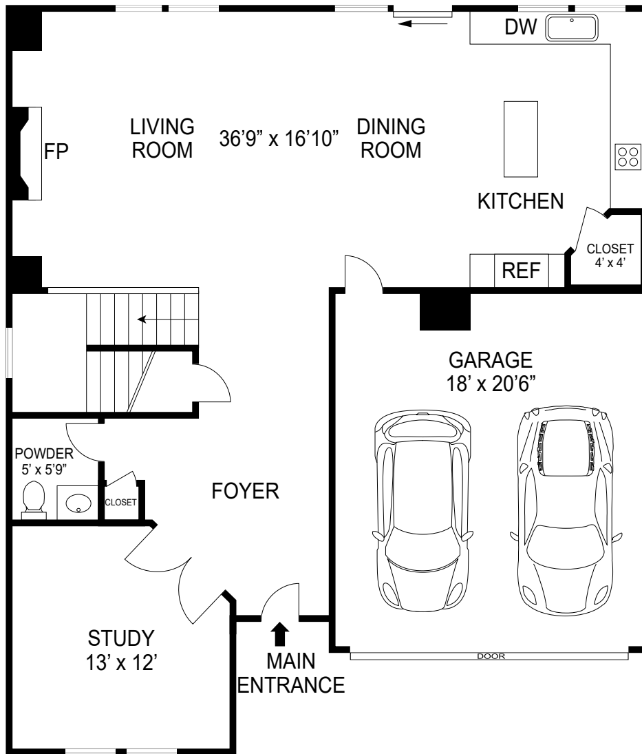
FIRST FLOOR 1044 sqf
