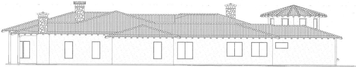
LEFT ELEVATION SCALE 1/4" = 1'-0"
